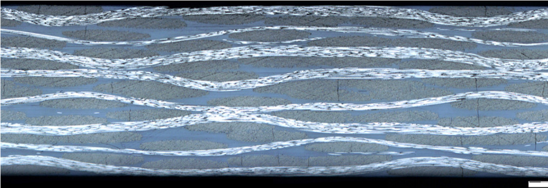
Ply level– Weft yarn damage on the surface layer (at the weft yarn centre)
