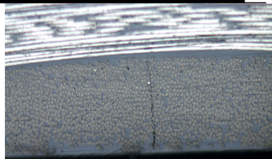
Damage location 3-1(Surface yarn) side view
