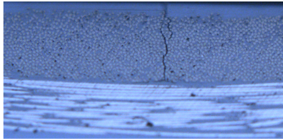
Ply level – Weft yarn damage at nested yarn configuration (at the edge of the weft yarn)
