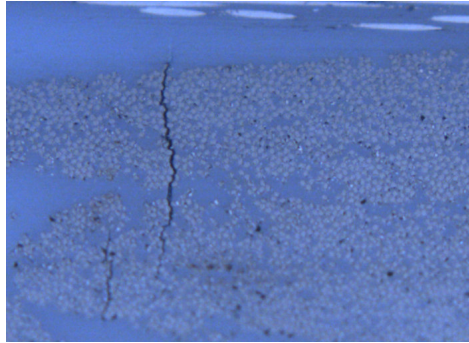
Micro level- fibre matrix debonding in the weft yarn
