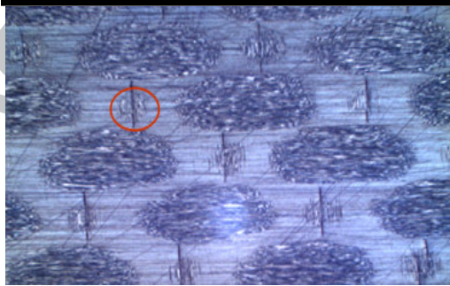
Damage location 3-1 (Surface yarn) top view
