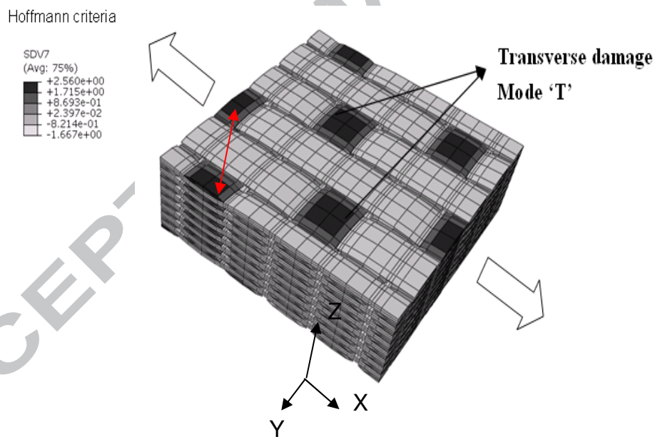
Figure 3. 8 unit cell stack FE analysis : a) Transverse stress distribution on the weft yarn; b) Transverse damage locations on the weft yarn at the yarn crimp location \langle 0.44\% \rangle with the 8 unit cell in-phase stack, in-plane PBC.
