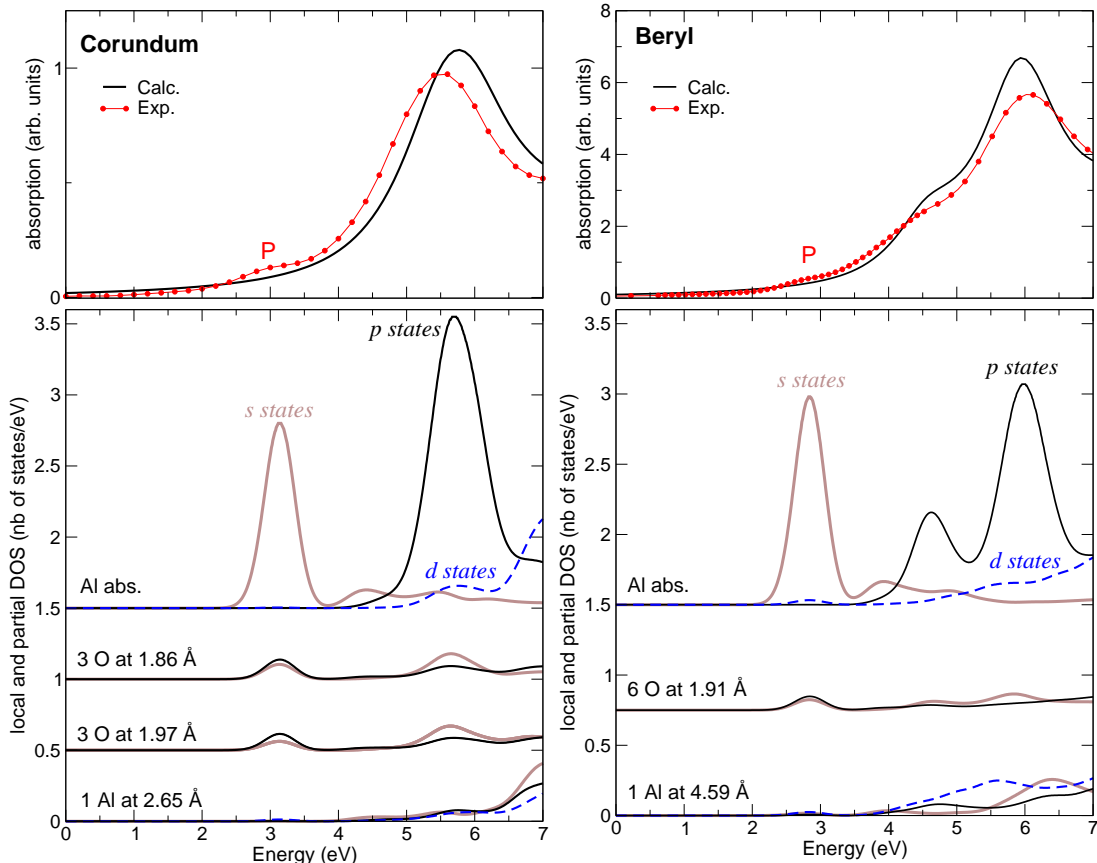
FIG. 5. Top: Calculated and experimental isotropic (2\sigma_{\perp} + \sigma_{\parallel})/3 spectra at the Al K -edge of corundum (left) and beryl (right). Bottom: partial and local density of states of corundum (left) and beryl (right) calculated for the supercell including a 1s core hole. The role of the Al 3s of the absorbing atom is prominent in the pre-edge region.
