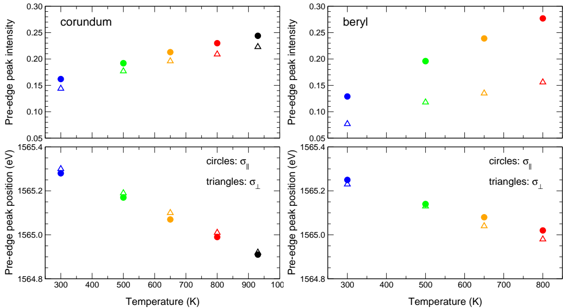
FIG. 4. Pre-edge intensity and energy position for both orientations and for both samples as a function of temperature. The y axis units of the upper panels are consistent with those of Fig. 2.
