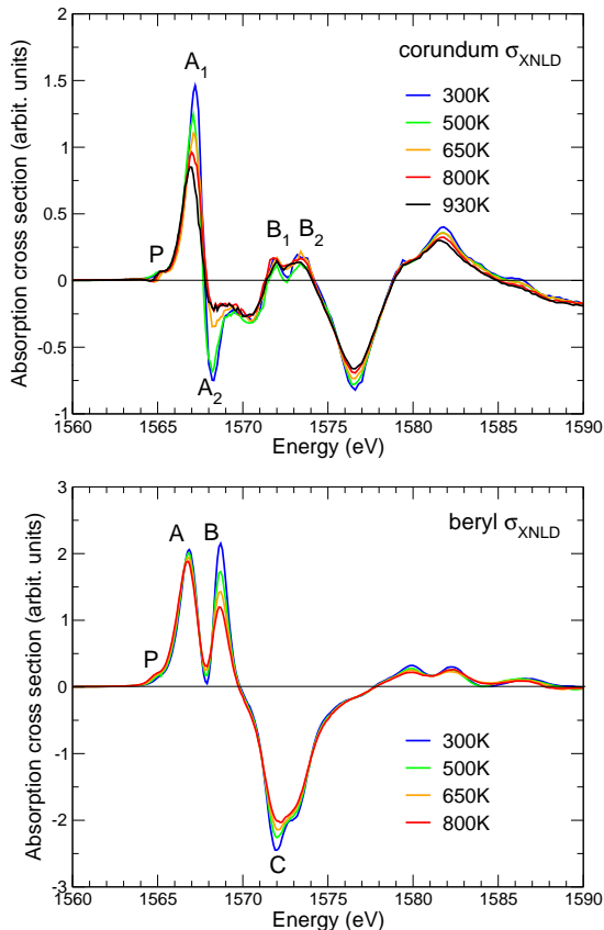
FIG. 3. Temperature dependence of the X-ray natural linear dichroism (XNLD) measured at the Al K -edge in corundum (top panel) and beryl (bottom panel). The cross section \sigma_{\text{XNLD}} is equal to the difference \sigma_{\parallel} - \sigma_{\perp} . Note that the y -axis range is twice larger for beryl than for corundum.
