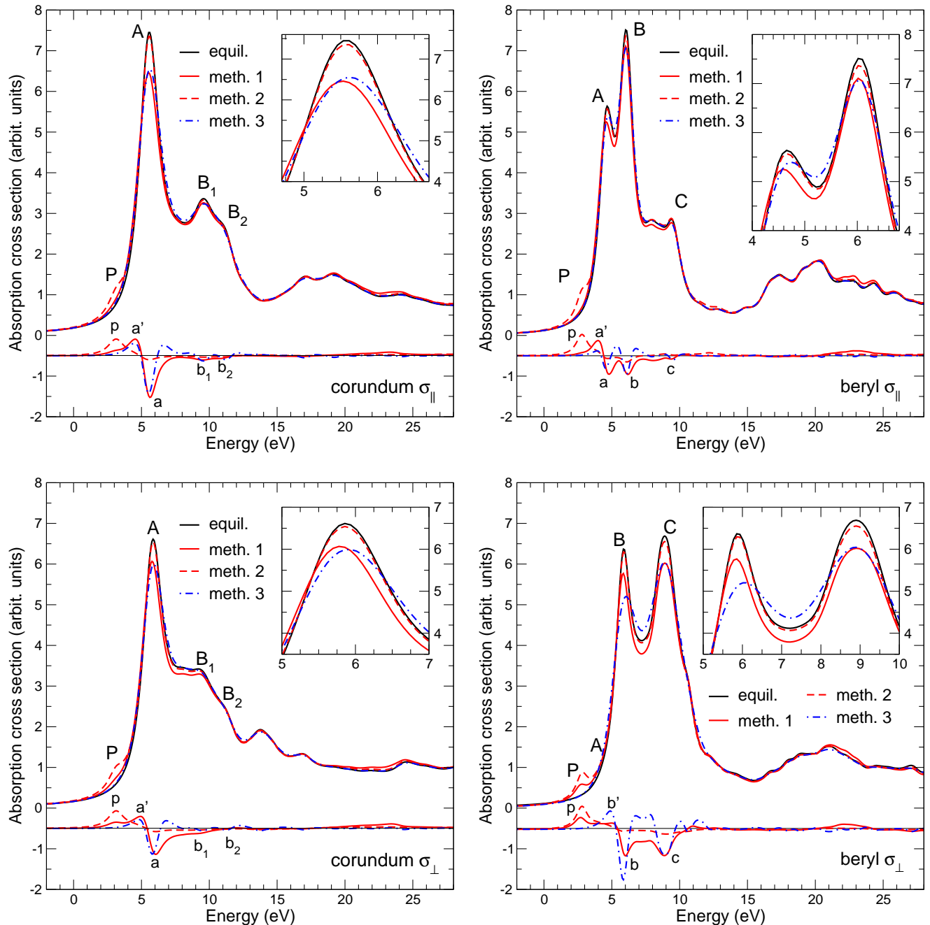
FIG. 6. Calculated \sigma_{\parallel} and \sigma_{\perp} spectra at the Al K edge of corundum (left) and beryl (right) along with difference of each spectrum with respect to the equil. reference. The ‘equil.’ spectra correspond to DFT calculation performed with the atoms at the equilibrium positions. The spectra labelled ‘meth. 1’, ‘meth. 2’ and ‘meth. 3’ refer to the three methods of vibration modeling described in section II. The upper-right inserts use the same legend code and present a zoom on the main peak(s).
