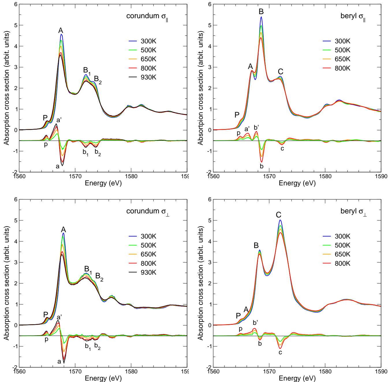
FIG. 2. Experimental X-ray absorption polarized spectra of corundum (left) and beryl (right) at the Al K -edge for different temperatures along with difference of each spectrum with respect to the 300K reference. The top and bottom panels display the \sigma_{\parallel} and \sigma_{\perp} spectra, respectively.
