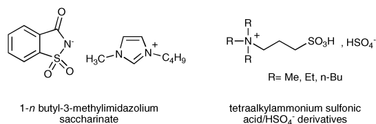
Fig. 1 Task-Specific Ionic Liquids (TSILs) used in MCRs.
