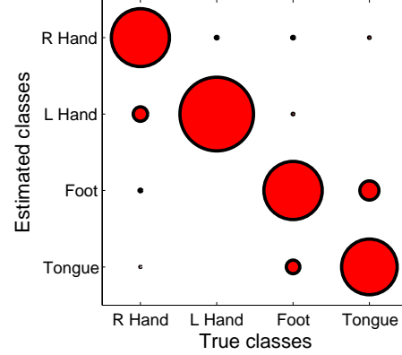
Figure 8. Confusion matrix in 30-fold cross validation for the subject S1
