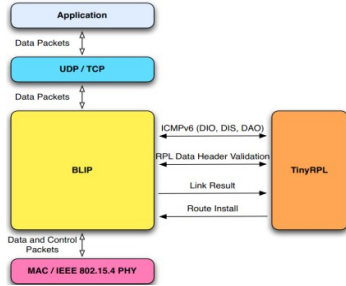
Figure 2. TinyRPL structure
