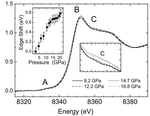
Figure 3: XANES spectra in YNiO_3 for selected representative pressures. A is the pre-edge, B the main edge structure and C the shoulder associated with middle range effects (see text). Lower inset : zoom on the C feature. Upper inset: maximum of the derivative at the edge as a function of the pressure.
