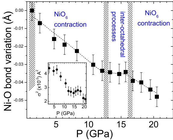
Figure 2: Pressure dependence of the average Ni-O bond length contraction \Delta R obtained from the EXAFS analysis. The line is just a guide for the eyes. Vertical lines separate different regions discussed in the text. Inset : \sigma^2 as a function of the pressure.
