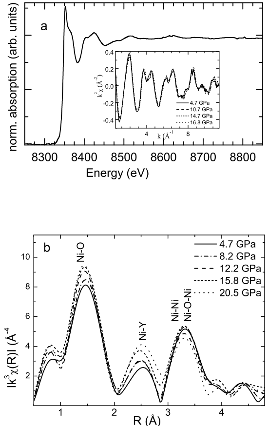
Figure 1: a: typical Ni K-edge XAS spectrum of YNiO_3 . Inset: EXAFS signal in the available k -range for different pressures. b Fourier transform modulus of the EXAFS oscillations for selected pressures.
