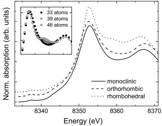
Figure 4: ab initio simulations of the XANES spectra for a Ni centered 61 atoms-cluster of YNiO_3 in the monoclinic (plain line), orthorhombic (dashed line) and LaNiO_3 -like rhombohedral (dotted line) structures. Inset : simulations for the rhombohedral structure and different cluster sizes .
