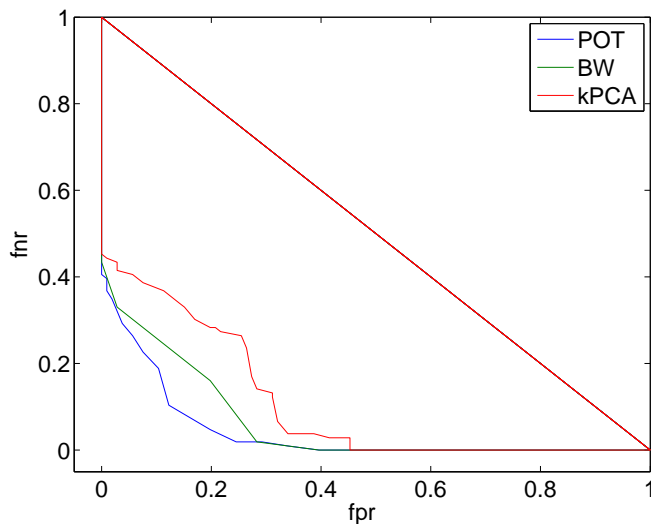
Figure 7: ROC curves for Algorithms POT, BW and kPCA. Faulty test data recorded after n = 2 days of operation.
