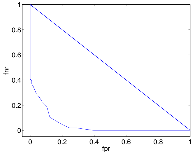
Figure 5: ROC curves for Algorithm POT. Faulty test data recorded after n = 2 days of operation.
