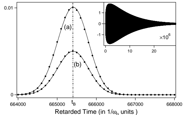
Figure 5: Brillouin precursor obtained in the Brillouin conditions, namely for \omega_c = 0.1 , \omega_p = 1.11 , \gamma = 0.0707 and \xi = 8.31 \times 10^5 (in \omega_0 units). For these parameters, \omega_0 t_B \approx 6.654 \times 10^5 and \beta \approx 1.78 \times 10^{-3} \omega_0 = 1.78 \times 10^{-2} \omega_c . Solid lines (bullets \bullet ) are the exact numerical solutions (the analytic solutions). Curve (a) is the precursor obtained with the canonical incident field \sin(\omega_c t) u_H(t) . The precursor of curve (b) is originated by the incident field e(0, t) = \sin(\omega_c t) [1 + \text{erf}(rt)] / 2 for r = \omega_c / 2\sqrt{2} . Inset: Sommerfeld precursor obtained in the conditions of curve (a). It fully vanishes in the conditions of curve (b).
