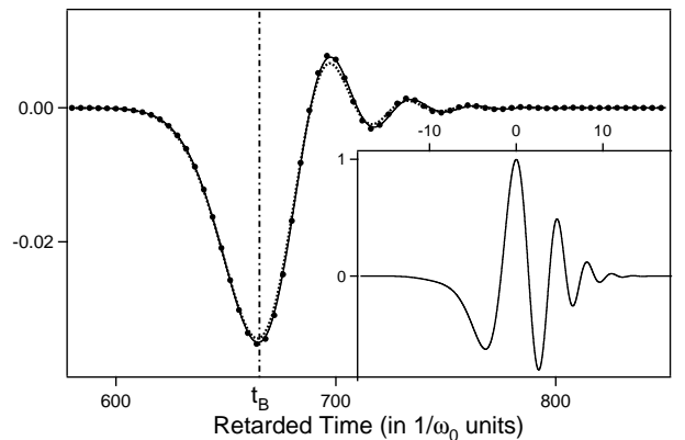
Figure 13: Brillouin precursor generated by a chirped incident pulse e^{-(t/T)^2} \cos(\omega_c t + \chi^2 t^2) , with T = 4\sqrt{2}/\omega_c and \chi = \omega_c/4 . The other parameters are as those of Fig.8 and Fig.12. The solid line, the bullets and the dashed line respectively are the exact numerical solution, the analytic solution derived from Eq.(43) and the approximate analytic solution of Eq.(48), obtained in the short pulse approximation. Inset: incident pulse. The corresponding Sommerfeld precursor has fully negligible amplitude ( 9 \times 10^{-11} !).
