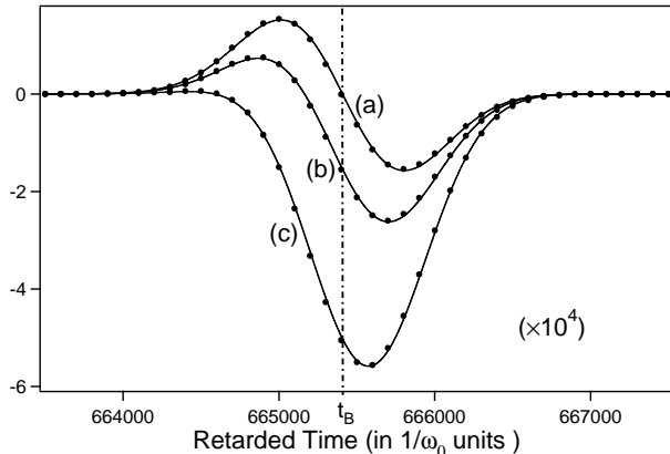
Figure 6: Brillouin precursor obtained with the incident fields (1 - e^{-rt}) \cos(\omega_c t) u_H(t) for (a) r \rightarrow \infty , (b) r = 65\omega_c and (c) r = 20\omega_c (solid lines). Other parameters as in Fig.5. The bullets \bullet correspond to the analytical solutions given by Eq.(27) or by the combination of this equation with Eq.(26).
