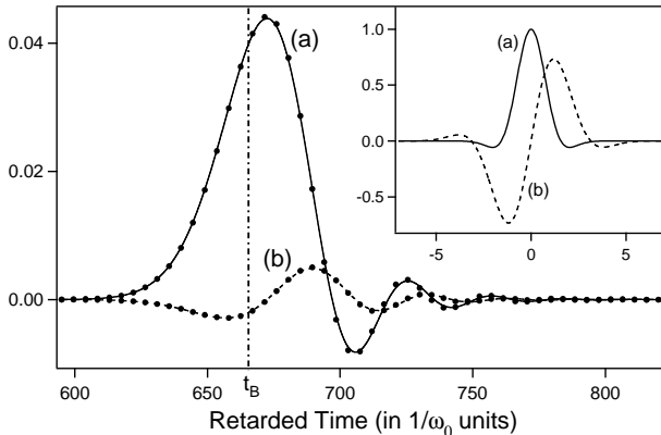
Figure 12: Brillouin precursors generated by the incident fields of Gaussian envelope (a) e^{-(t/T)^2} \cos(\omega_c t) with T = \sqrt{2}/\omega_c and (b) e^{-(t/T)^2} \sin(\omega_c t) with T = \sqrt{6}/\omega_c . The parameters are those of Fig.8. In both cases, the pulse duration has been chosen in order to maximize the precursor amplitude (see text). The solid and dashed lines are the exact numerical solutions whereas the bullets are the analytical solutions obtained in the short pulse approximation [Eq.(45) and Eq.(46)], indiscernible from those obtained without approximation [Eq.(43)]. Inset: corresponding incident fields. Numerical calculations shows that the Sommerfeld precursors generated by these fields have negligible amplitudes, respectively (a) 5.6 \times 10^{-7} and (b) 1.15 \times 10^{-10} .
