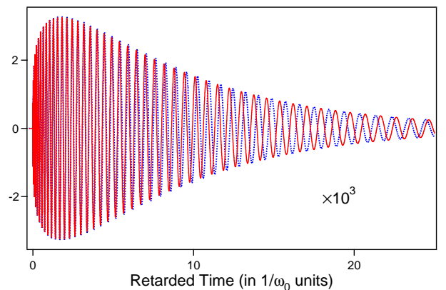
Figure 3: Sommerfeld precursor originated by the canonical incident field \sin(\omega_c t)u_H(t) . The solid (dashed) line is the exact numerical solution (the approximate analytic solution). Parameters as in Fig.2.
