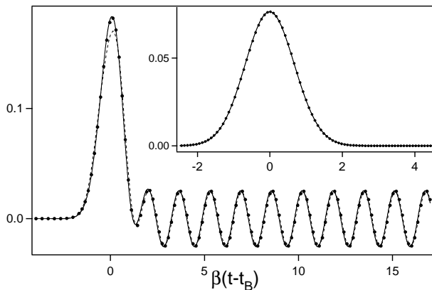
Figure 7: Brillouin precursor and main field obtained for \omega_c \approx 3.84\beta as a function of \beta(t - t_B) . The solid line, the bullets \bullet and the dashed line are respectively the exact numerical solution, the analytical solution given Eq.(29) and its approximate form given Eq.(30). Inset: Brillouin precursor obtained for \omega_c \approx 7.67\beta . The two analytical solutions are undistinguishable in this case and the amplitude of the main field is negligible.
