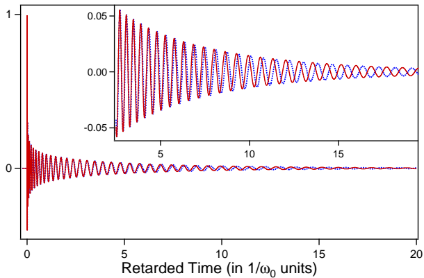
Figure 2: Sommerfeld precursor originated by the incident field \cos(\omega_c t)u_H(t) . The solid (dashed) line is the exact numerical solution (the approximate analytic solution). Parameters (in \omega_0 units) : \omega_c = 1 , \omega_p = 1.11 , \gamma = 0.0707 and \xi = 831 . Inset : enlargement of the tail of the precursor.
