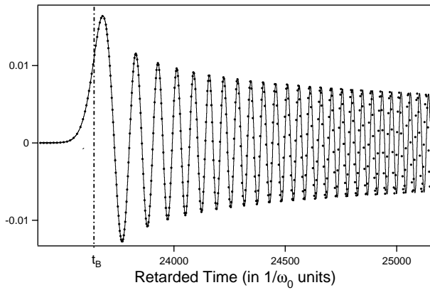
Figure 10: Brillouin precursor in the dispersion dominant limit. The solid line (bullets \bullet ) is the exact numerical solution (the analytical solution). Parameters (in \omega_0 units): \omega_c = 0.836 , \omega_p = 1.11 , \gamma = 10^{-4} and \xi = 2.95 \times 10^4 , leading to \omega_0 t_B \approx 2.3641 \times 10^4 , b \approx 0.0257\omega_0 and \beta \approx 0.252\omega_0 . The carrier frequency \omega_c is at the lower boundary of the opacity region [ \alpha(\omega_c)z \approx 20 ].
