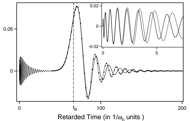
Figure 9: Comparison of the Brillouin precursor obtained outside the asymptotic limit (solid line) with the analytical forms given Eq.(34) ( \bullet ) and Eq.(36) (dashed line). Parameters (in \omega_0 units): \omega_c = 1 , \omega_p = 1.11 , \gamma = 0.0707 and \xi = 83.1 , leading to \omega_0 t_B \approx 66.54 , b \approx 0.182 \omega_0 and \beta \approx 0.178 \omega_0 . Inset: corresponding Sommerfeld precursor (solid line) compared to the analytic form given Eq.(21) (dashed line).
