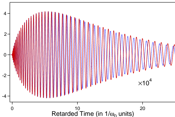
Figure 4: Sommerfeld precursor originated by the incident field e(0, t) = \tanh(rt) \sin(\omega_c t) u_H(t) . The solid (dashed) line is the exact numerical solution (the approximate analytic solution) obtained for r = \omega_0 . Other parameters as in Fig.2.
