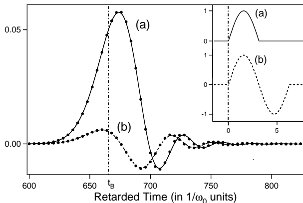
Figure 11: Comparison of the Brillouin precursors e'_B(z, t) generated by an incident square-modulated field of duration (a) T = T_c/2 and (b) T = T_c . The parameters are those of Fig.8. The solid and dashed lines are the exact numerical solutions, indiscernible from the analytical solutions given by Eq.(37). The bullets are the approximate solutions (a) 2e_B(z, t - T_c/4) and (b) T_c e_B(z, t - T_c/2) . As expected the precursor amplitude for T = T_c/2 is twice that attained with a step-modulated field (see Fig.8) whereas that attained for T = T_c is much smaller. Inset: corresponding incident fields.
