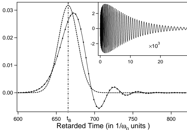
Figure 8: Brillouin precursor obtained in the simple asymptotic limit with the canonical incident field \sin(\omega_c t)u_H(t) . Parameters (in \omega_0 units): \omega_c = 1 , \omega_p = 1.11 , \gamma = 0.0707 and \xi = 831 , leading to \omega_0 t_B \approx 665.4 , b \approx 8.44 \times 10^{-2} \omega_0 and \beta \approx 5.64 \times 10^{-2} \omega_0 . The solid line, the bullets \bullet and the dashed line are respectively the exact numerical solution, the analytical solution given Eq.(34) and the Gaussian that would be obtained in the dominant-attenuation approximation. The conditions are those of Fig.3. The corresponding Sommerfeld precursor is given in inset for reference.
