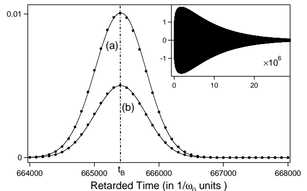
Figure 5: Brillouin precursor obtained in the Brillouin conditions, namely for \omega_c = 0.1 , \omega_p = 1.11 , \gamma = 0.0707 and \xi = 8.31 \times 10^5 (in \omega_0 units). For these parameters, \omega_0 t_B \approx 6.654 \times 10^5 and \beta \approx 1.78 \times 10^{-3} \omega_0 = 1.78 \times 10^{-2} \omega_c . Solid lines (bullets \bullet ) are the exact numerical solutions (the analytic solutions). Curve (a) is the precursor obtained with the canonical incident field \sin(\omega_c t) u_H(t) . The precursor of curve (b) is originated by the incident field e(0, t) = \sin(\omega_c t) [1 + \text{erf}(rt)] / 2 for r = \omega_c / 2\sqrt{2} . Inset: Sommerfeld precursor obtained in the conditions of curve (a). It fully vanishes in the conditions of curve (b).
