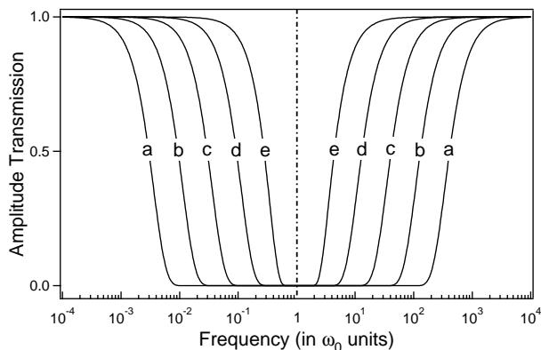
Figure 1: Amplitude transmission |H(z, \omega)| of the medium as a function of the frequency modulus |\omega| (logarithmic scale). Parameters (in \omega_0 units) : \omega_p = 1.11 , \gamma = 0.0707 and \xi = 8.31 \times 10^5 for the curve (a) corresponding to the Brillouin choice ( z = 10^{-2} \text{ m} ). The curves (b), (c), (d) and (e) are obtained for propagation distances (and thus \xi ) respectively 10, 100, 1 000 and 10 000 times smaller.
