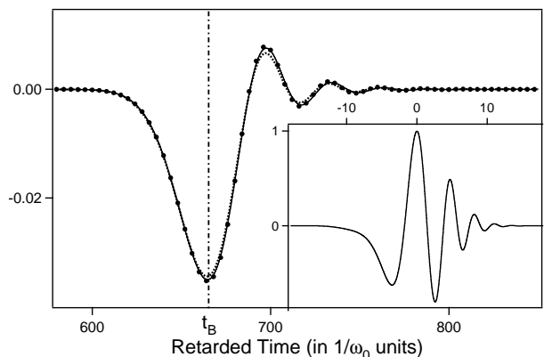
Figure 13: Brillouin precursor generated by a chirped incident pulse e^{-(t/T)^2} \cos(\omega_c t + \chi^2 t^2) , with T = 4\sqrt{2}/\omega_c and \chi = \omega_c/4 . The other parameters are as those of Fig.8 and Fig.12. The solid line, the bullets and the dashed line respectively are the exact numerical solution, the analytic solution derived from Eq.(43) and the approximate analytic solution of Eq.(48), obtained in the short pulse approximation. Inset: incident pulse. The corresponding Sommerfeld precursor has fully negligible amplitude ( 9 \times 10^{-11} !).
