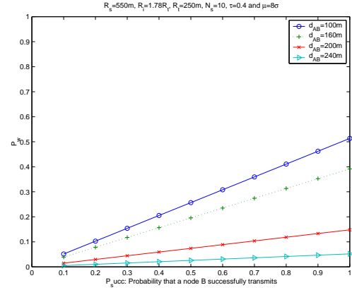
Fig. 8. P_w versus distance between two nodes ( \tau = 0.4 and \mu = 8.\sigma )
