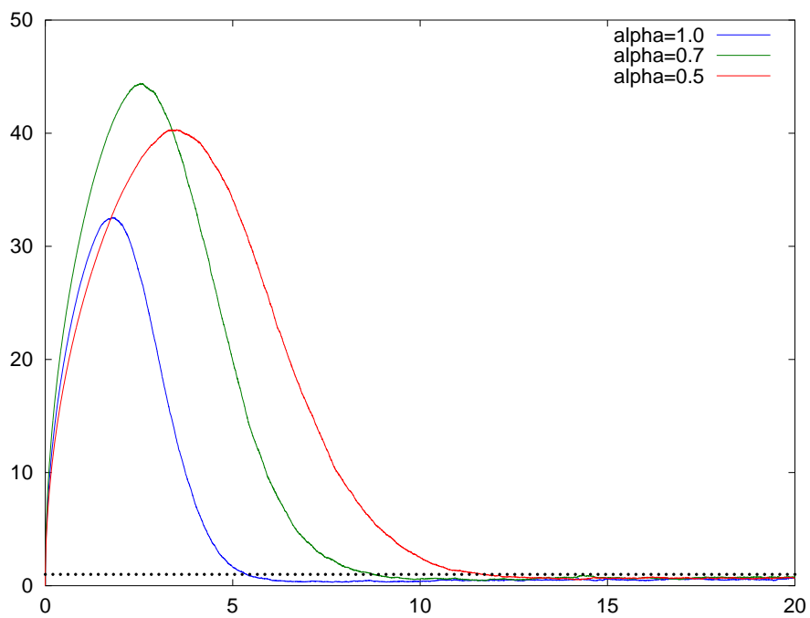
Figure 2: Convergence of \frac{2\alpha\sqrt{2}}{\varepsilon\sqrt{1+\alpha^2}}\sqrt{t} \mathbb{E}(|b| - \mu_t \cdot b) with \mu_0 = -b , |b| = 1 and \varepsilon = 0.1 . The horizontal dashed line is at level one. The expectation is computed using a Monte-Carlo method with 100 samples.
