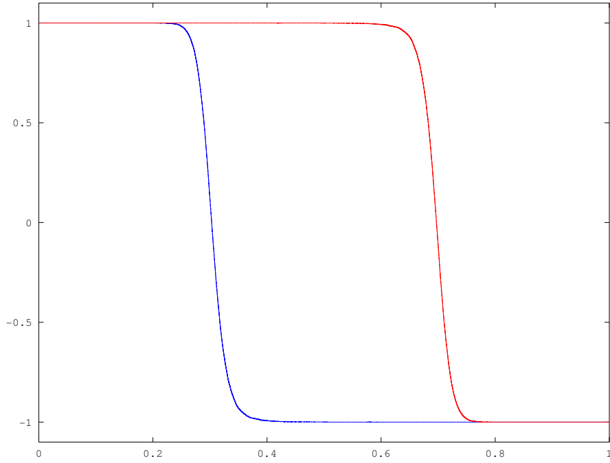
Figure 3: Pathwise hysteresis phenomena with \alpha = 1 , \varepsilon = 0.005 and \eta = 0.01 . The red curve is the forward path whereas the blue curve is the backward path. The x -axis is time.
