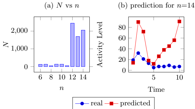
Figure 8: Study of the epidemic threshold for the diffusion of an information about Google in the first network
