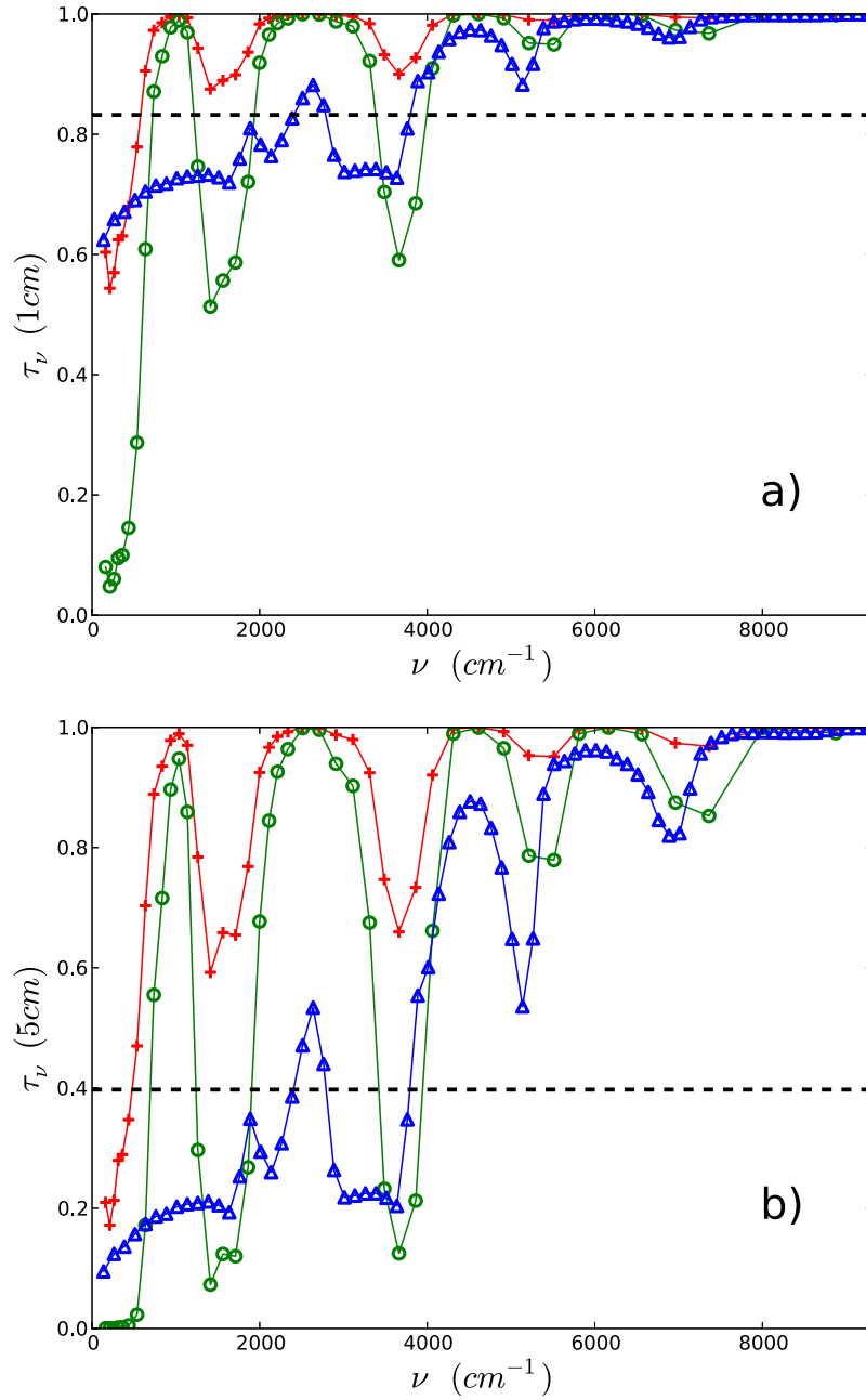
Figure 7: Transmissivity of columns of lengths 1\text{cm} (a) and 5\text{cm} (b) associated with interfaces (dashed line), water droplets at (R_d = 25 \mu\text{m}, f_v = 10^{-3}) ( \Delta ), steam at temperature T_v = 1000 \text{ K} and pressure p_v = 1 \text{ atm} ( \times ) or p_v = 5 \text{ atm} ( \circ ).
