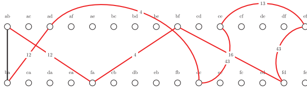
Fig. 3. The incompatibility graph associated with the sub-matrix from Figure 1 (Right). Every edge is labeled with the corresponding row except the edge (ab, ba) which represents an edge of first type. Note that for the cycle we need all rows and all columns from the sub-matrix from the Table 1. This odd-length cycle gives a certificate that the sub-matrix does not have the SC1P.
