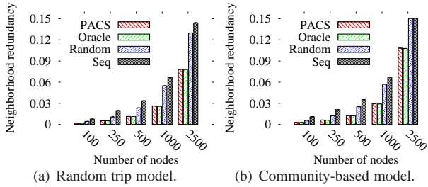
Figure 11: Neighborhood redundancy. Dissemination of a 48MB file divided into 128 pieces of 384kB. Area 1,000m \times 1,000m . PACS limits neighborhood redundancy as compared to sequential and random strategies.
