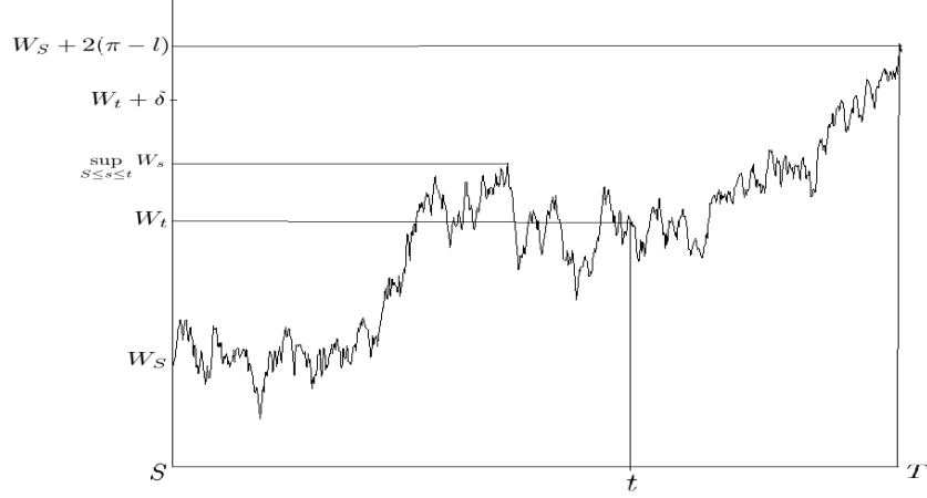
Figure 2: The path of W after S .
