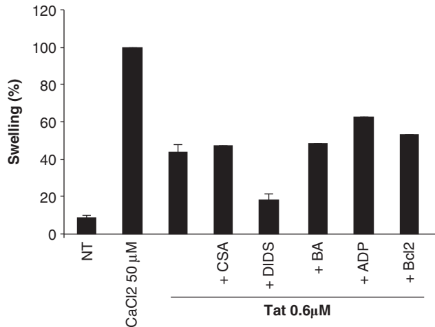
Figure 3 Tat-induced swelling in heart-isolated mitochondria. Isolated mouse heart mitochondria were exposed to full-length Tat[1-86] 0.6 \mu M and mitochondrial swelling (measured as 90° light scattering at 545 nm) was monitored for 30 min. When indicated, mitochondria were preexposed for 5 min in the presence or absence of the following compounds: cyclosporin A (CsA; 30 \mu M), ADP (1 mM), bongkreik acid (BA; 50 \mu M), Bcl-2 (400 nM), or DIDS (5 \mu M). Then, mitochondria were incubated with Tat[1-86] (0.3 \mu M; 30 min). Percentages of mitochondrial swelling (left panel) were calculated as described under Materials and Methods. Positive control was defined by the addition of 50 \mu M CaCl 2 . Histograms represent mean values ( \pm S.D.) of three independent experiments
