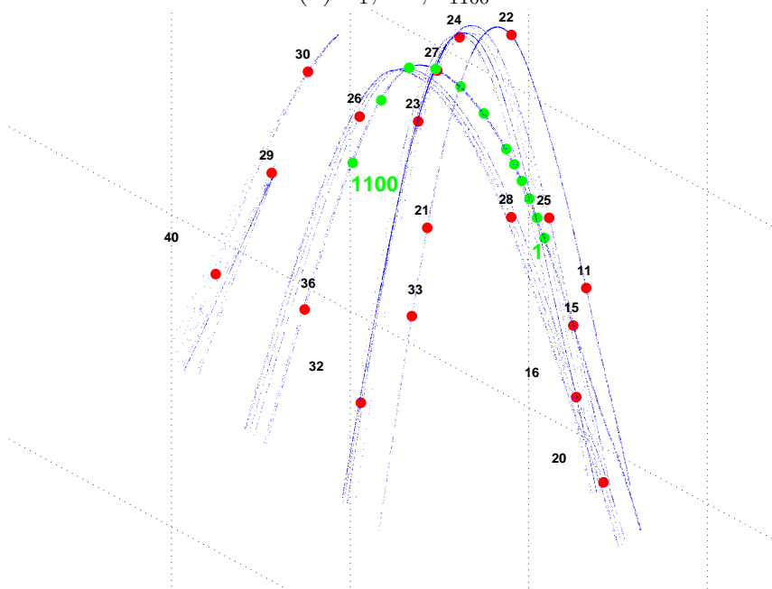
(b) T^2(x_1), \dots, T^2(x_{1100})
