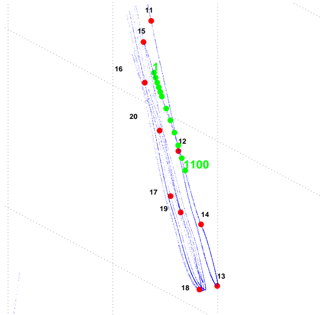
(a) x_1, \dots, x_{1100}
