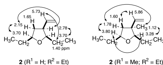
Figure 1. Selected NOE interactions for the determination of the relative configuration of 2 ( \text{R}^1 = \text{H} , \text{R}^2 = \text{Et} ) and 2 ( \text{R}^1 = \text{Me} , \text{R}^2 = \text{Et} ).
