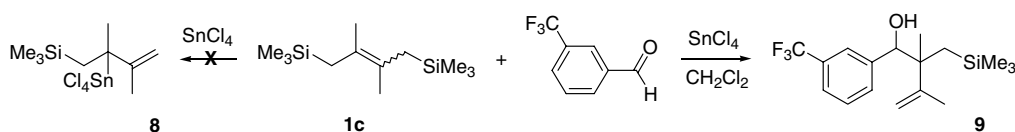
Scheme 4. Addition of 1c to m -trifluoromethylbenzaldehyde.
