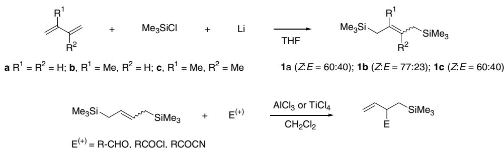
Scheme 1. Synthesis of 1,4-bis(trimethylsilyl)-2-butenes 1a-c from 1,3-dienes and addition of 1a to various electrophilic reagents.
