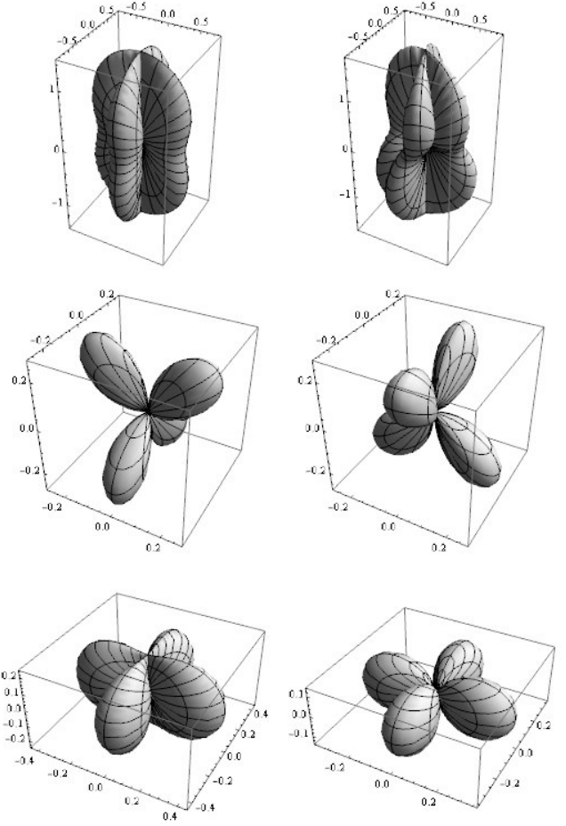
Figure 3: Plots along the panel lines from left to right of angular pattern functions of a detector for each polarization. From left plus mode F_+ , cross mode F_\times , B mode F_B , C mode F_C , D mode F_D , and scalar mode F_s . The angular pattern function of the F_B and F_C mode is the same except for a rotation.
