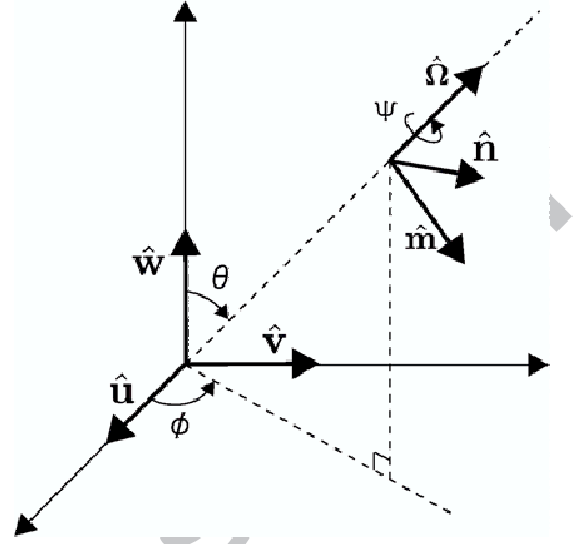
Figure 2: The coordinate systems used to calculate the polarization tensors and the pictorial view of the coordinate transformation.
