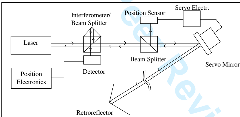
Figure 2 – Interferometry in Laser Trackers (Estler WT et al, 2002).
