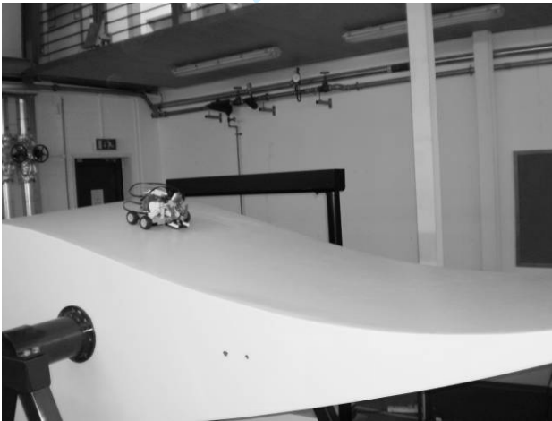
Figure 11 - The robot carrying out scanning operation
