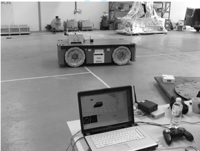
Figure 16 – Full-scale omniMove moving to waypoint under iGPS guidance
