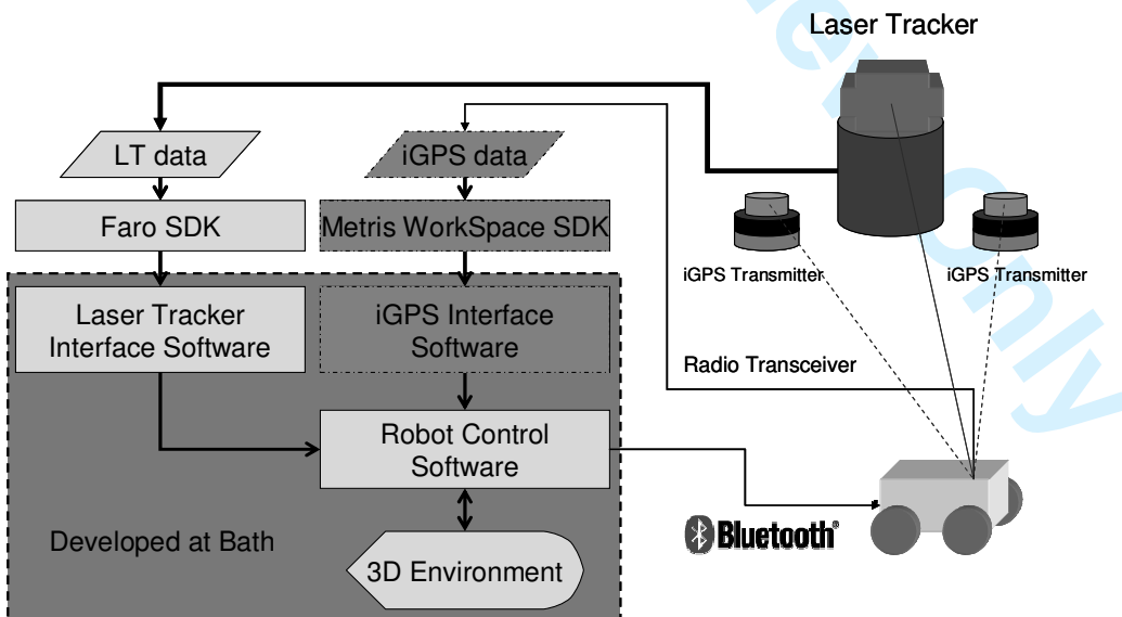
Figure 6 – Software system
