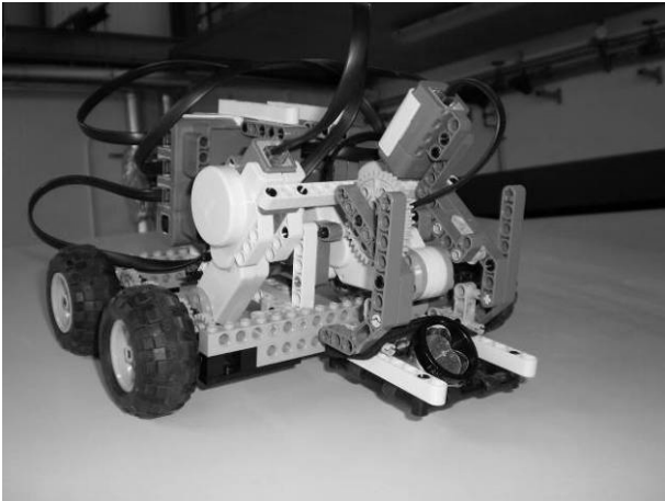
Figure 4 – Mobile robot carrying a laser tracker SMR
