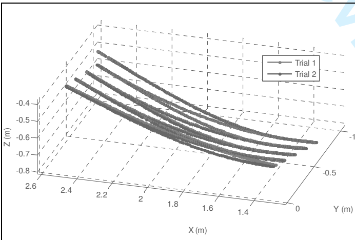
Figure 12 - Scanned data points
