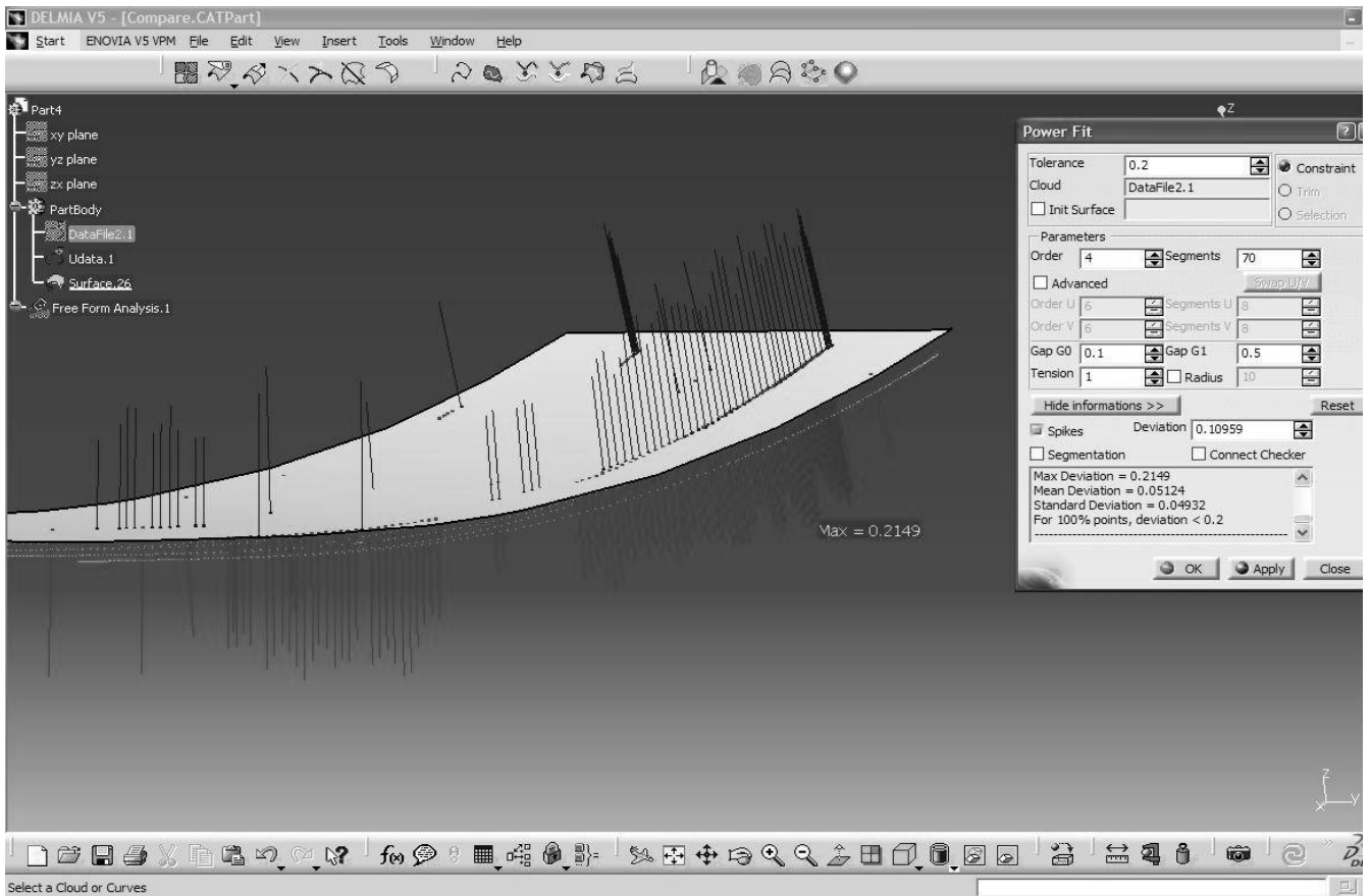
Figure 13 - Best fitting a NURBS surface to the scanned data in CATIA V5
