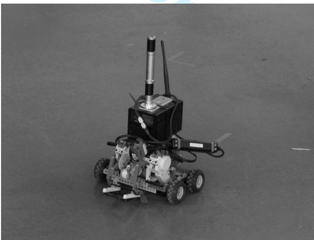
Figure 5 - Mobile robot carrying an iGPS vector bar
