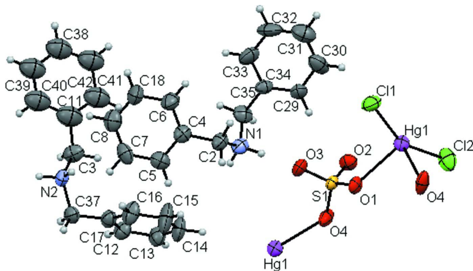
Figure 1 Molecular structure of the title compound. Displacement ellipsoids are drawn at the 50% probability level.
