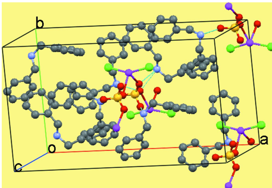
Figure 2 Molecular packing viewed along the c axis. H atoms have been omitted for clarity.
