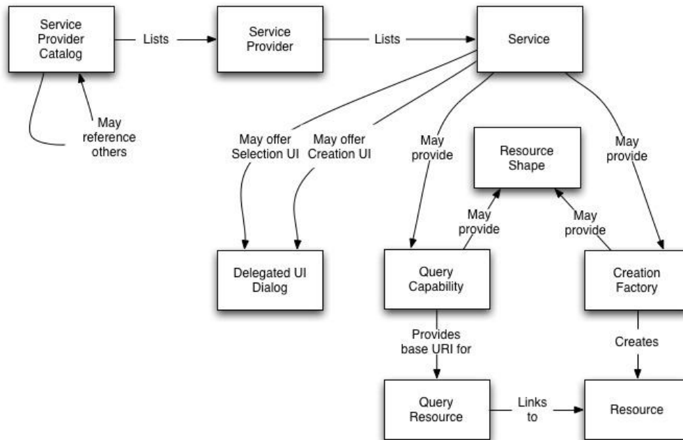
Fig. 1: OSLC Core Specification concepts and relationships
