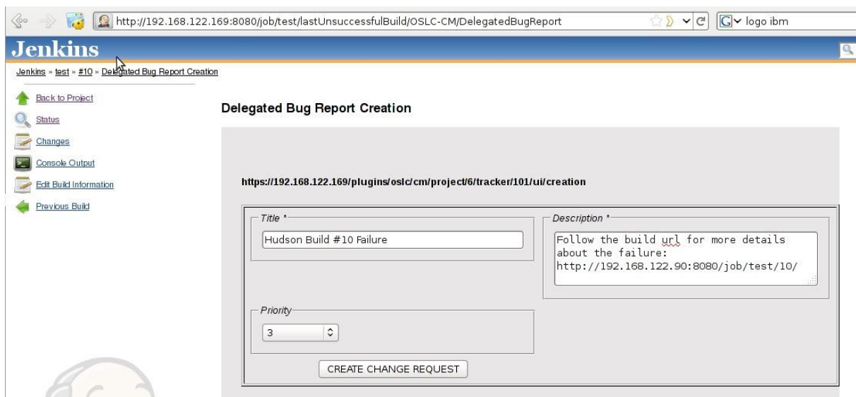
Fig 2: Jenkins and FusionForge mashup
