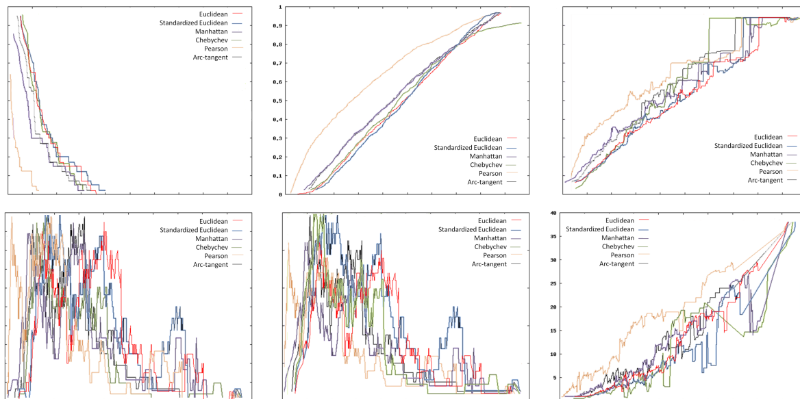
Figure 4. Comparative analysis of sporulation data with different distances. Percentage of isolated vertices - Density - Variance - Number of CMSs - Number of non-trivial atoms - Average size of overlaps
