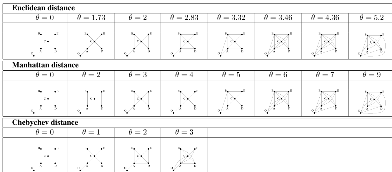
Figure 3. Impact of the distance function on our example data set.
