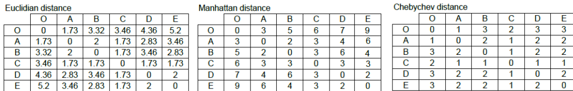
Figure 2. Effect of the distance function on dissimilarity values of a data set.
