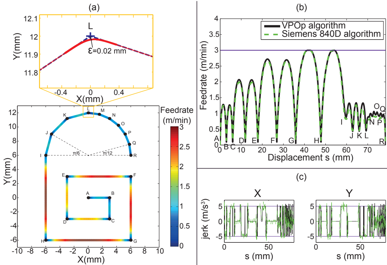
Figure 7: (a) lock tool path, (b) feedrate profile, (c) jerk constraints verification
