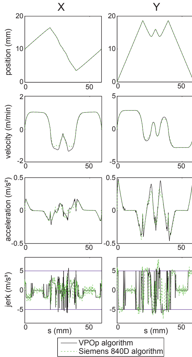
Figure 6: Trident - constraints verification.
