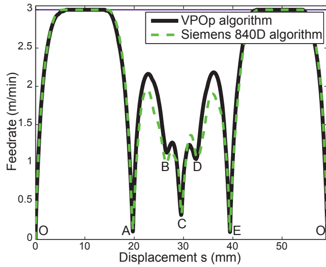
Figure 5: Trident - feedrate.
