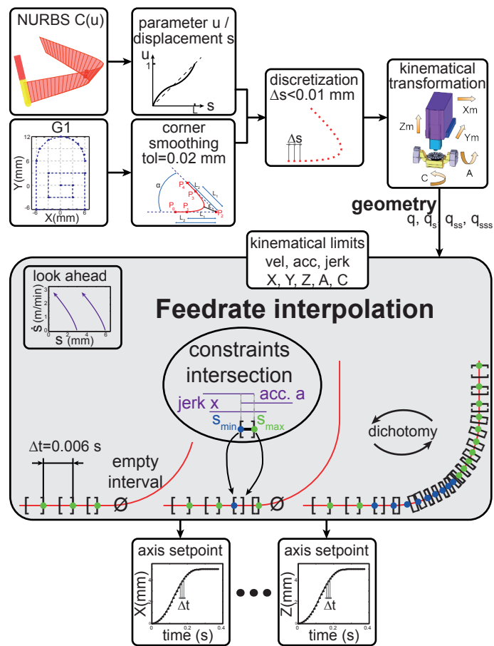
Figure 1: VPOp algorithm
