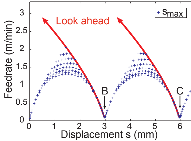
Figure 8: Look ahead for the lock.
