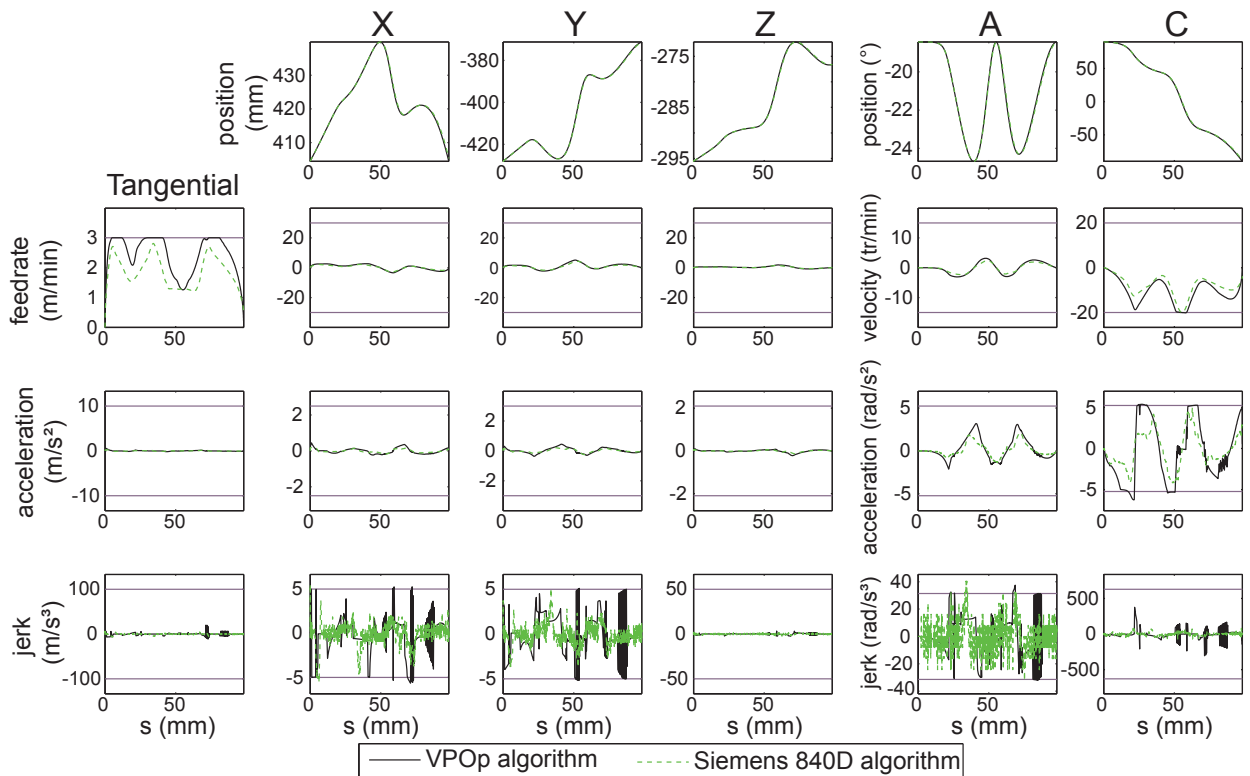
Figure 10: Open pocket - constraints verification on the 5-axis machine.
