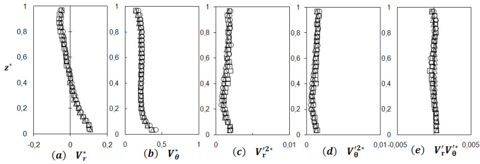
Figure 2: Experimental results at r^* = 0.976 . Shrouded rotor system: \circ \lambda = 0 ; \square \lambda = 0.27 ; Unshrouded rotor system: \triangle \lambda = 0.27 .
