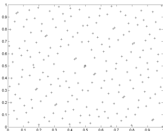
(c) Sequence of Sobol.
