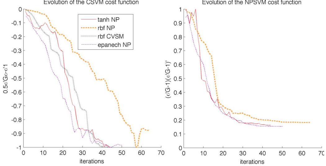
Figure 2: Evolution of the cost function during training. Curves are scaled on vertical axis. On the left, we report the value of the usual CSVM cost function during training. On the right are curves corresponding to the modified cost function that is actually minimized. While the standard CSVM cost function decreases monotonically ( rbf CSVM on the left graph), the cost function for NPSVM may increase. Note that test performance are similar for each of the reported experiment on this figure (dataset is synthetic data generated from the apple/banana setting).
