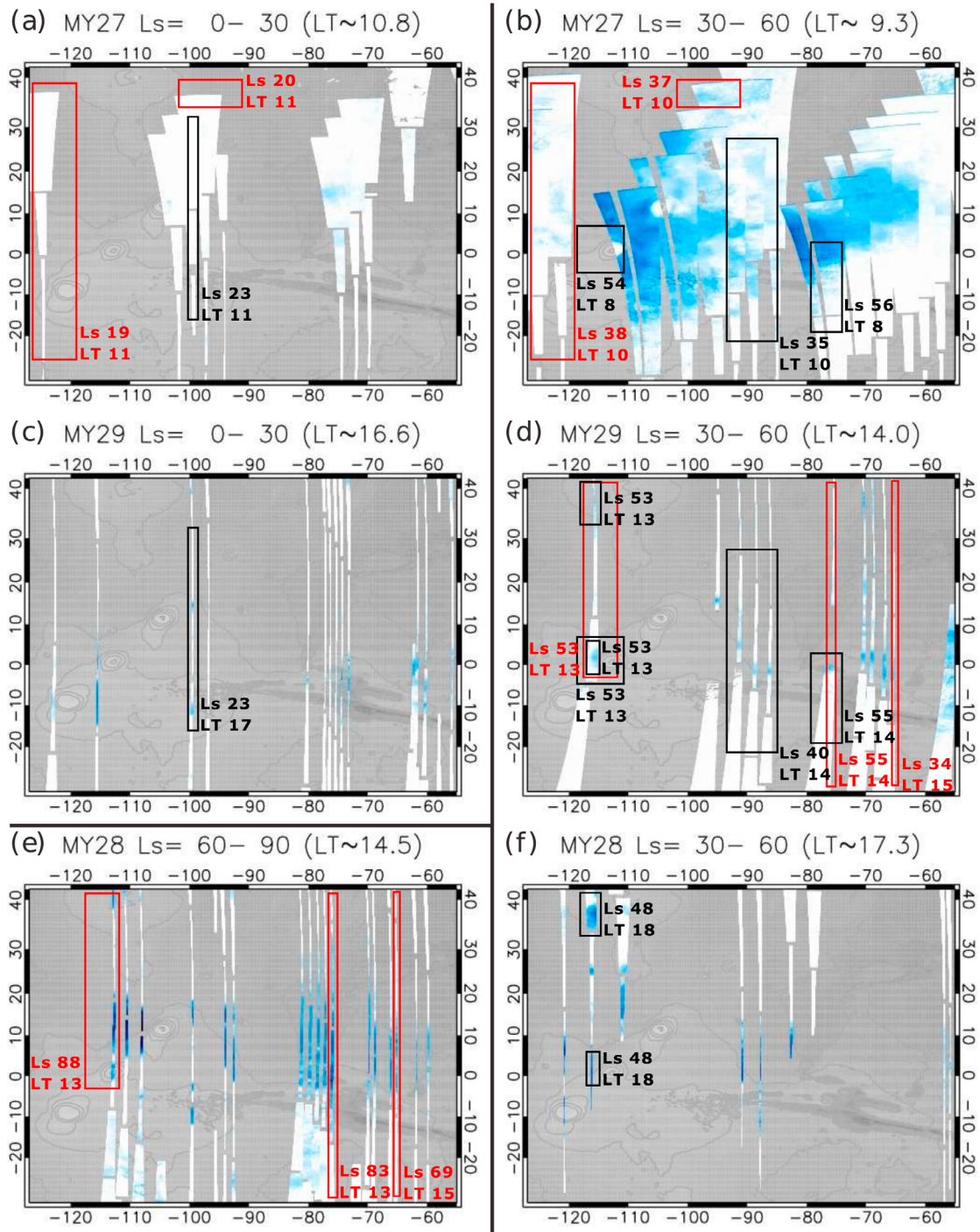
Figure 1. Cloud index maps (see section 3) for intervals of 30^\circ of L_s . Diurnal variations can be appreciated between Figures 1a and 1c for the L_s = 0\text{--}30^\circ period, and between Figures 1b, 1d, and 1f for the L_s = 30\text{--}60^\circ period. Only one set of observations is available for the L_s = 60\text{--}90^\circ period (Figure 1e). Red boxes indicate the regions that were observed at different L_s but at the same local time LT (less than one hour difference) from one year to another. On the contrary, black boxes show particular regions that were observed at different local times but at the same L_s (less than 5^\circ difference). For all the maps presented in this paper, the background grey scale is the MOLA (Mars Orbiter Laser Altimeter) topography [Zuber et al. , 1992].
