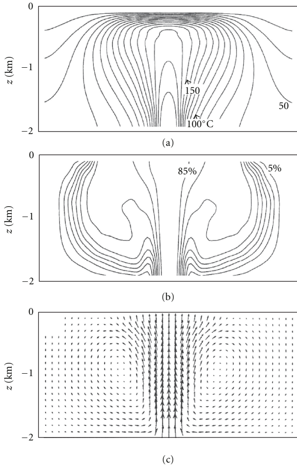
FIGURE 5: Results of reservoir simulation: natural-state distributions of (a) temperature (contour interval 10°C), (b) mass fraction of “source fluid”, and (c) fluid mass flux. Earth-surface SP distributions computed by the so-called “EKP postprocessor” for this natural state (solid curve), and for a subsequent exploited state (broken curve), are shown in (d), after [57].
