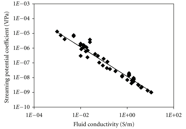
FIGURE 4: Streaming potential coefficient from data collected (in absolute value) on sands and sandstones at pH 7-8 (when available) from Ahmad [100]; Li et al. [67]; Jouniaux and Pozzi [101]; Lorne et al. [86]; Pengra et al. [102]; Guichet et al. [21]; Perrier and Froidefond [103]; Guichet et al. [88]; Ishido and Mizutani [96]; Jaafar et al. [98]. The regression (black line) leads to C_{s0} = -1.2 \times 10^{-8} \sigma_f^{-1} . A zeta potential of -17 \text{ mV} can be inferred from these collected data from Allègre [24].
