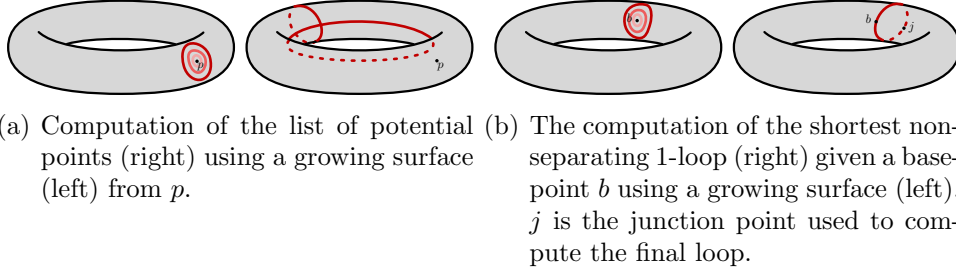
Figure 7: Two steps of the non-separating 1-loop computation.
