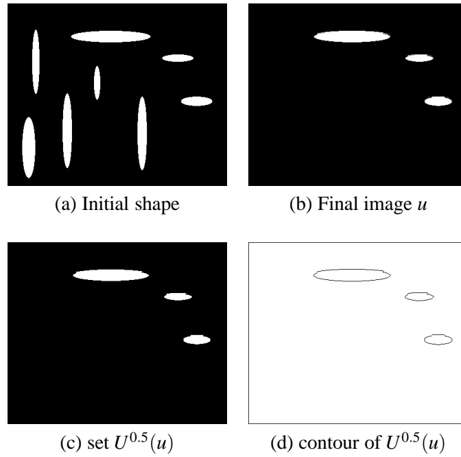
Figure 17: Experimental results of geometrical filtering (selection of horizontal ellipses) with UBR ( r = 20, \lambda = 0.05, \varepsilon_{up} = 0.0001 ) for the image “ellipses”. We show the initial image (a), the final image without thresholding (b) the set U^{0.5}(u) (c) and its boundary (d).
