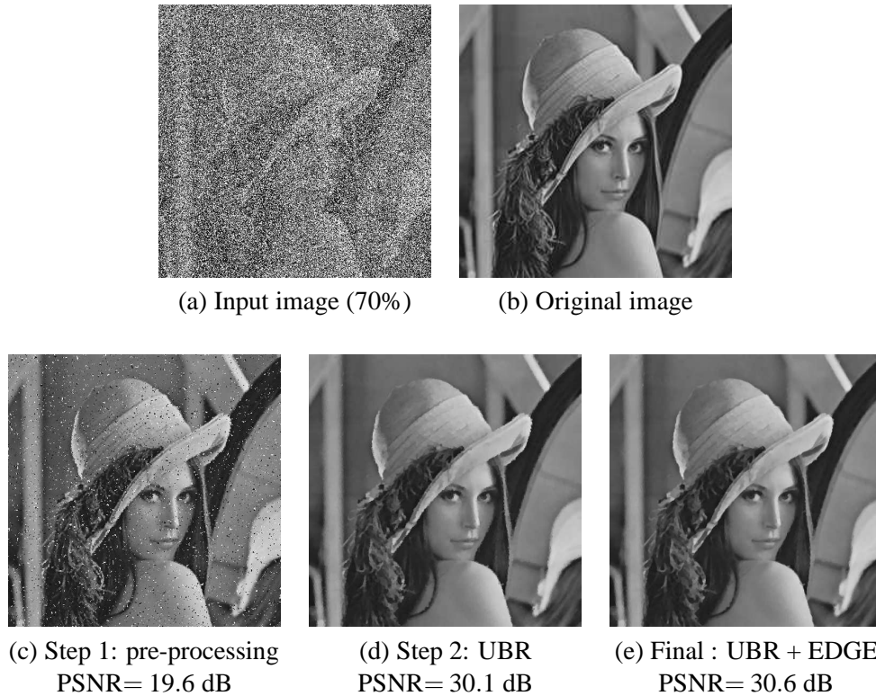
Figure 8: Salt and pepper noise removal using the algorithm UBR-EDGE for the image Lena corrupted by a noise of 70%. The result is given for each step of the process. The image obtained after the pre-processing (median+mean) is given in (c). This image is used as an input of the algorithm UBR and the result is given in (d). A last post-processing is applied to the image which yields to the final result given in (e).
