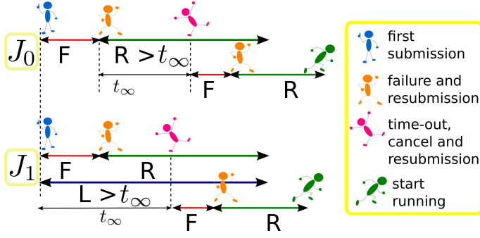
Figure 2. Two ways of taking faults into account in the resubmission strategy J_0 (with time-out adapted dynamically in case of failures) and J_1 (with fixed time-out, independently of failures).
