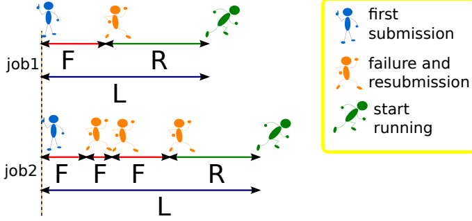
Figure 1. Two examples of job submission with resubmissions in case of failures.
