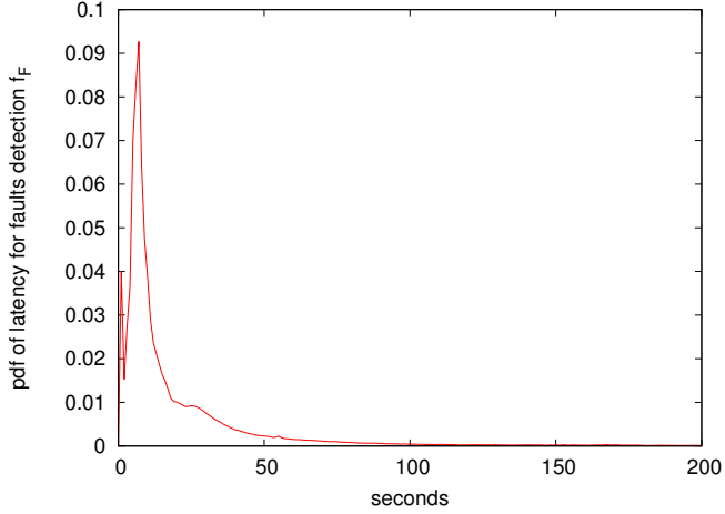
Figure 5. Probability density function of the latency for fault detection. We observe a maximum at 7 seconds.
