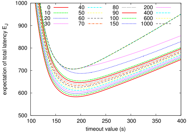
Figure 8. Translating pdf of failure detection latency: impact on E_{J_0} . Both optimal time-out value and expectation of total latency are varying. For translation higher than 200 seconds, results are similar since the optimal time-out is lower than 200 seconds.
