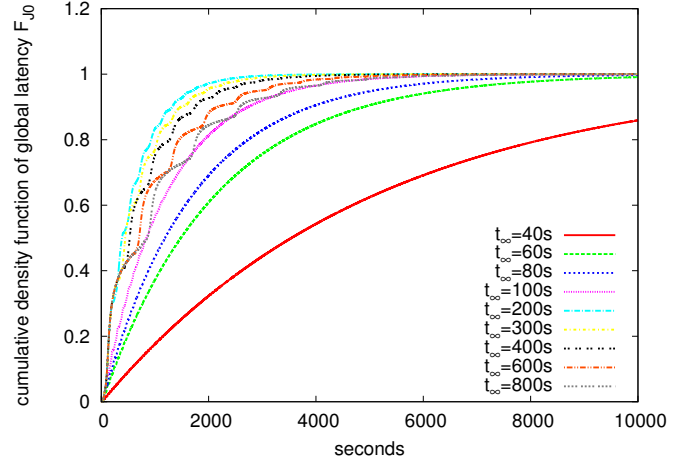
Figure 3. Strategy J_0 . Cumulative density functions of global latency including resubmission for different time-out values ( t_\infty ).
