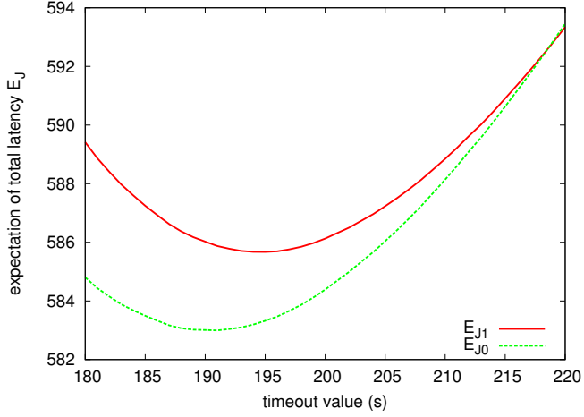
Figure 6. Zoom on the expectation of total latency for strategies J_0 and J_1 .
