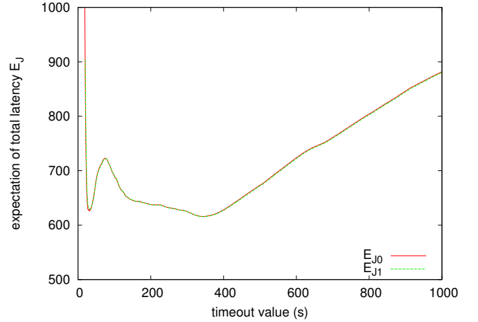
Figure 9. 2010 data. Expectation of execution time including resubmissions for strategies J_0 and J_1 : results are very similar even if the profile differs from the one obtained with older data (see for example figure 4).
