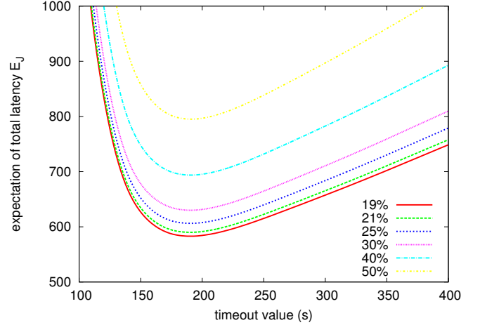
Figure 7. Varying the ratio of faults \phi in case of J_0 . The optimal time-out value does not vary while the expectations of total latency are increasing.
