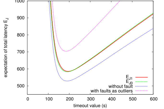
Figure 4. Expectation of total latency with respect to the time-out value t_\infty : cases of strategy J_1 , strategy J_0 , a simple model ignoring failures and an approximation where failures are accounted as outliers.
