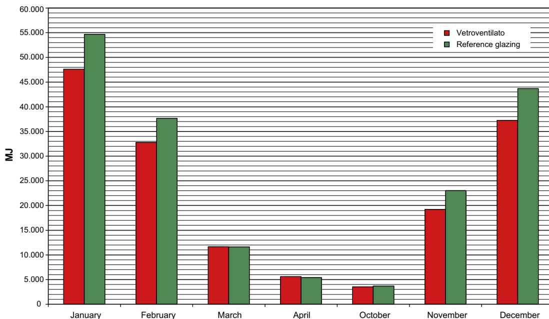
Fig. 12. Monthly net heating energy demand for the case study concerning the office building located in Milan.
