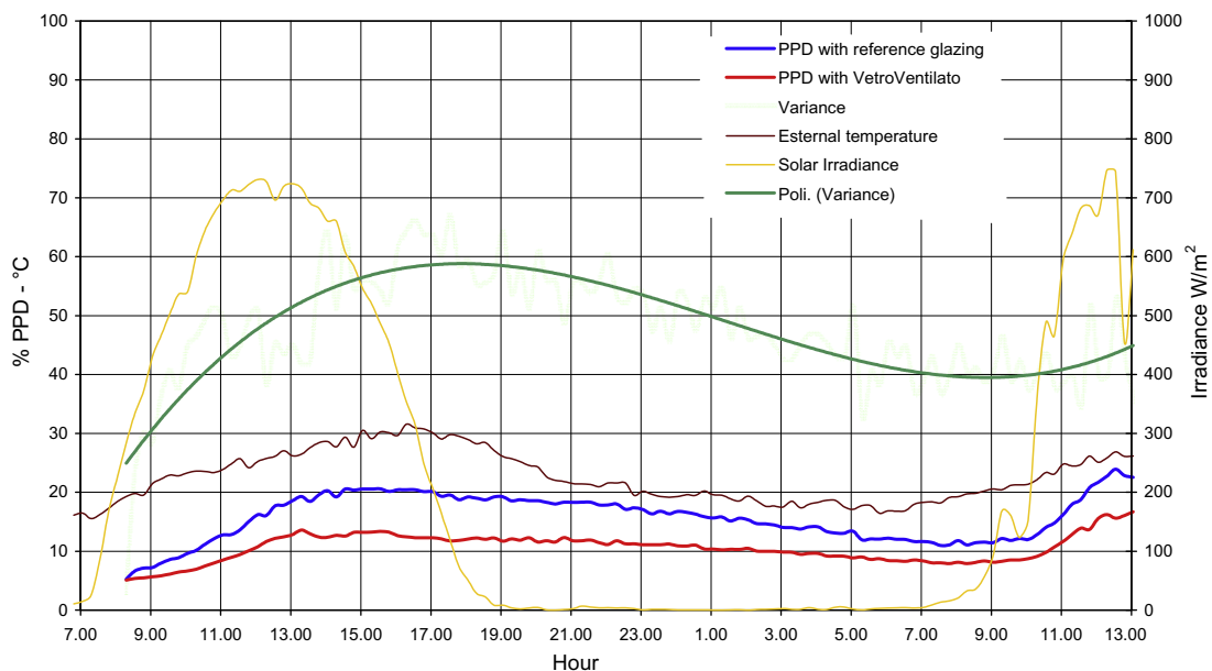
Fig. 6. PPD comparison in a typical summer day – slat angle of the shading component \alpha = 60^\circ and \Delta T = 2^\circ\text{C} .
