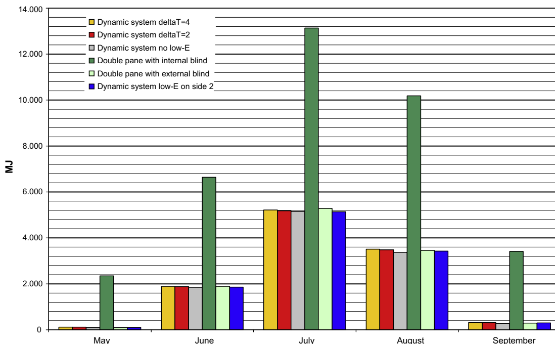
Fig. 9. Predicted monthly cooling energy need for the restaurant case study.
