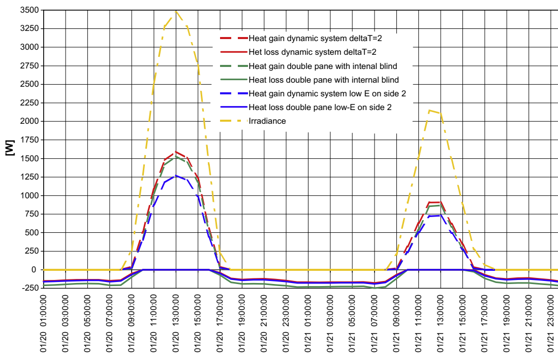
Fig. 10. Hourly winter heat gain and loss – south facing of the restaurant case study.
