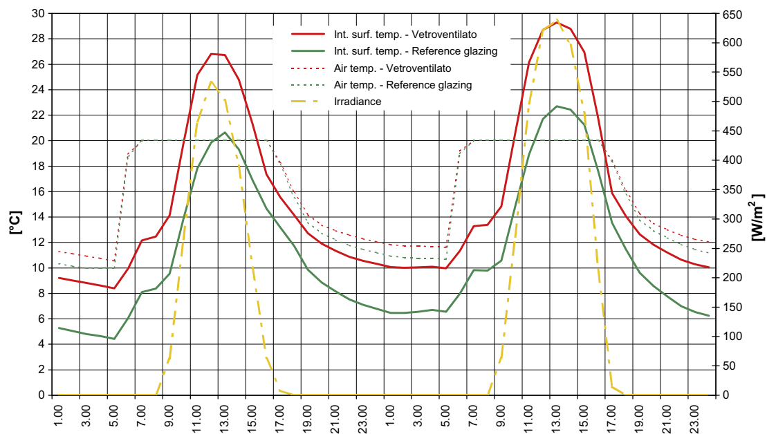
Fig. 15. Hourly surface temperatures for the south front and indoor air (temperature) in winter conditions for the office building case study located in Milan.
