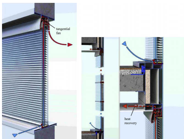
Fig. 1. To the left: the dynamic system operating in heat push out mode (airflow internal/external); to the right: the dynamic system integrated in a curtain wall (airflow internal/internal).
