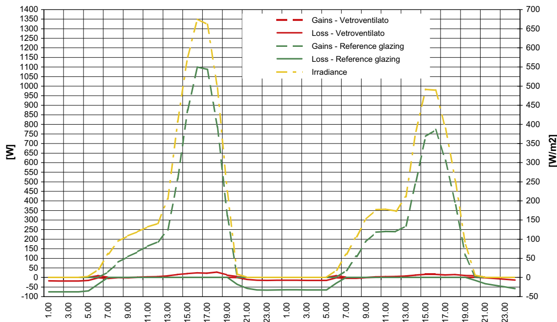
Fig. 14. Hourly solar gains vs loss for the west front of the case study concerning the office building located in Milan.
