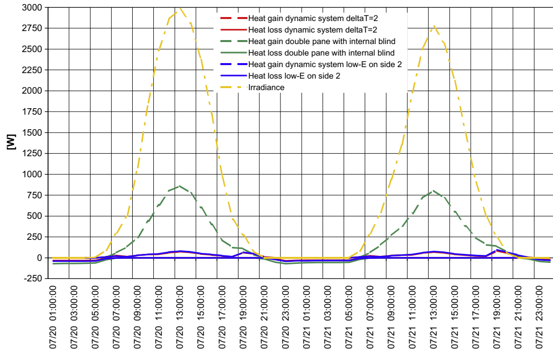
Fig. 11. Hourly summer heat gain and loss – south facing of the restaurant case study.
