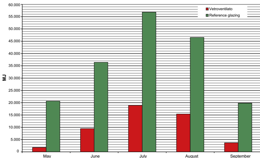
Fig. 13. Monthly net cooling energy demand for the case study concerning the office building located in Milan.
