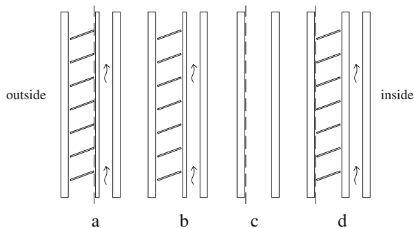
Fig. 3. (a) Dynamic system, (b) dynamic system no low- E , (c) double pane low- E and (d) dynamic system low- E on side 2.
