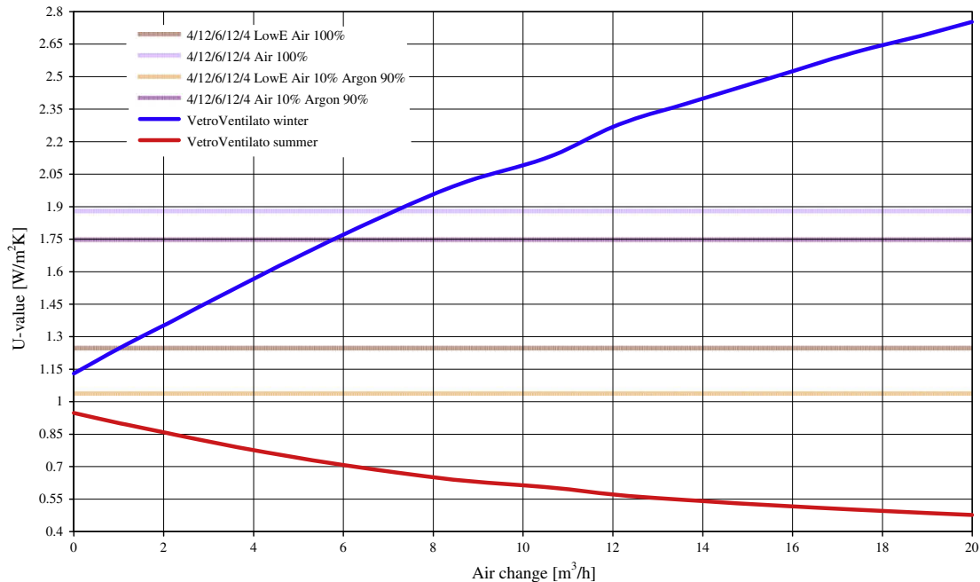
Fig. 7. U -value pattern depending on the air change per hour.
