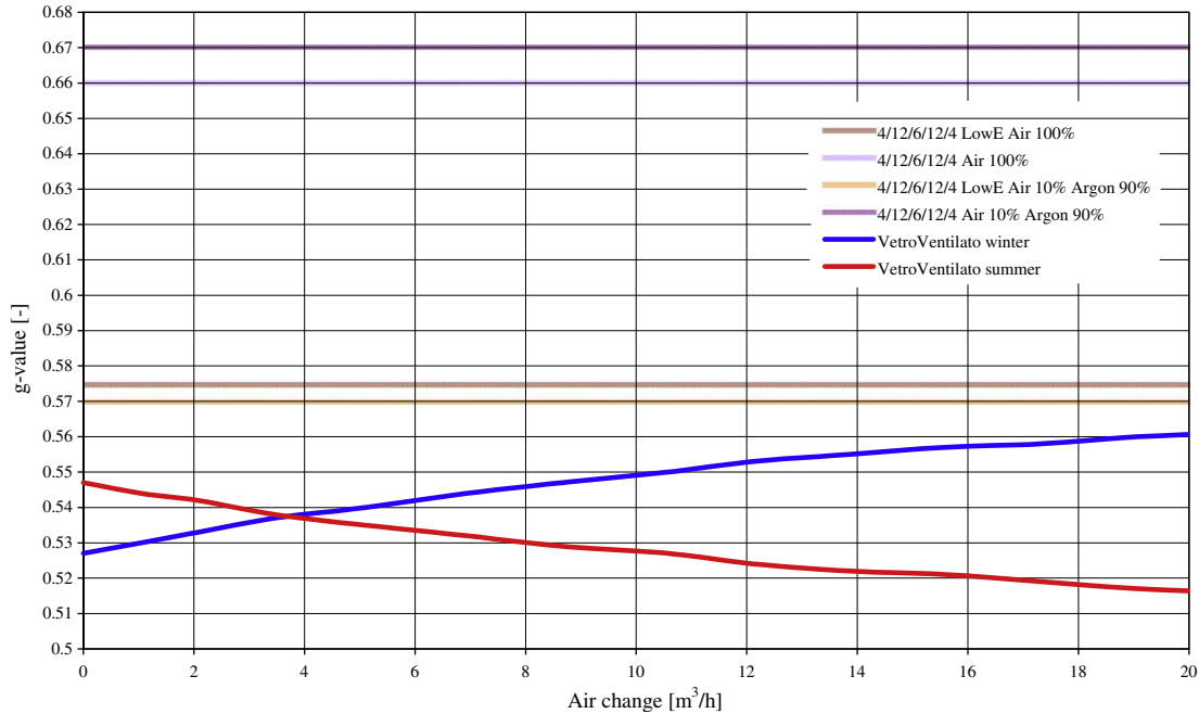
Fig. 8. g -value pattern depending on the air change per hour.
