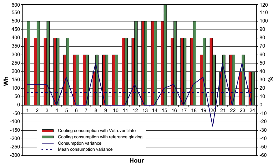
Fig. 5. Electrical consumption in a typical summer day.
