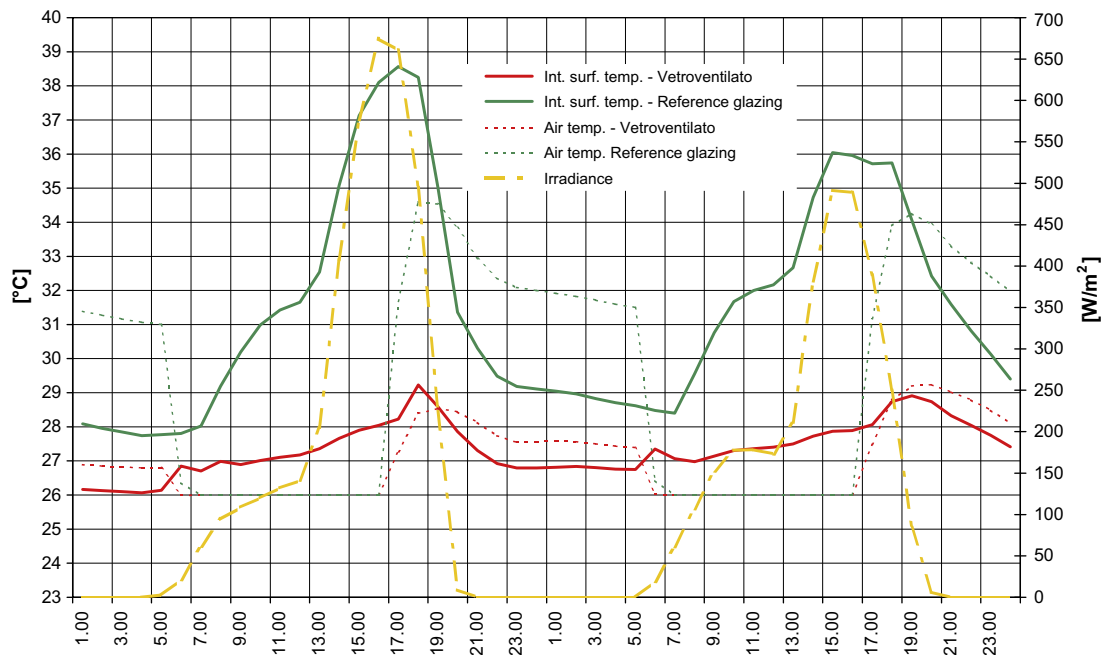
Fig. 16. Hourly surface temperatures for the south front and the internal air temperature in summer conditions for the case study concerning the office building located in Milan.
