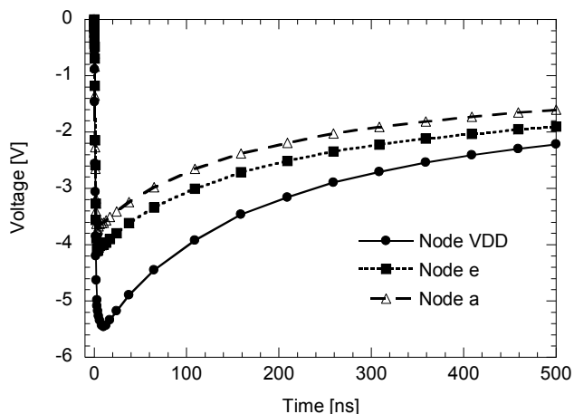
Figure 6: 1 kV HBM simulations of the circuit in Figure 4 without reverse diode D_1 . HBM stress was applied negative between V_{DD} and V_{SS} .
