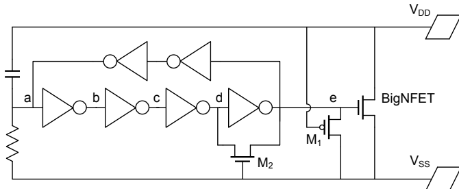
Figure 9: Schematic of symmetric RC-triggered FinFET power clamp based on Figure 7. The addition of M_2 further improves the turn-on voltage during negative stress events.
