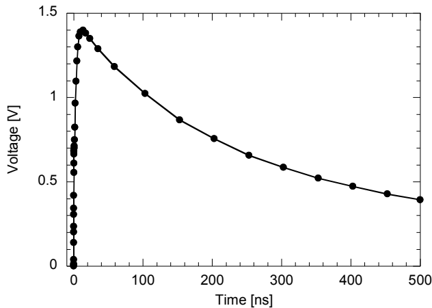
Figure 5: 1 kV HBM simulations of the circuit in Figure 4. HBM stress was applied positive between V_{DD} and V_{SS} .
