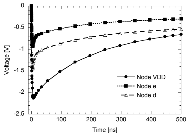
Figure 8: 1 kV HBM simulations of the circuit in Figure 7. HBM stress was applied negative between V_{DD} and V_{SS} .
