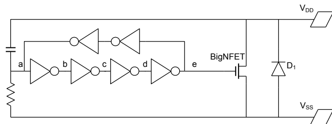
Figure 4: Schematic of RC-triggered power clamp. The addition of inverters and feedback relaxes the constraint on the RC-network.
