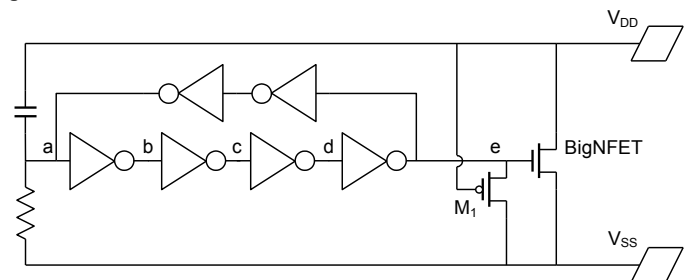
Figure 7: Schematic of symmetric RC-triggered FinFET power clamp. The addition of M_1 enables the BigNFET to operate in active mode also during negative stress events.
