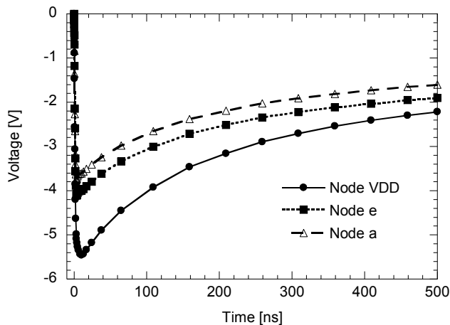
Figure 6: 1 kV HBM simulations of the circuit in Figure 4 without reverse diode D_1 . HBM stress was applied negative between V_{DD} and V_{SS} .
