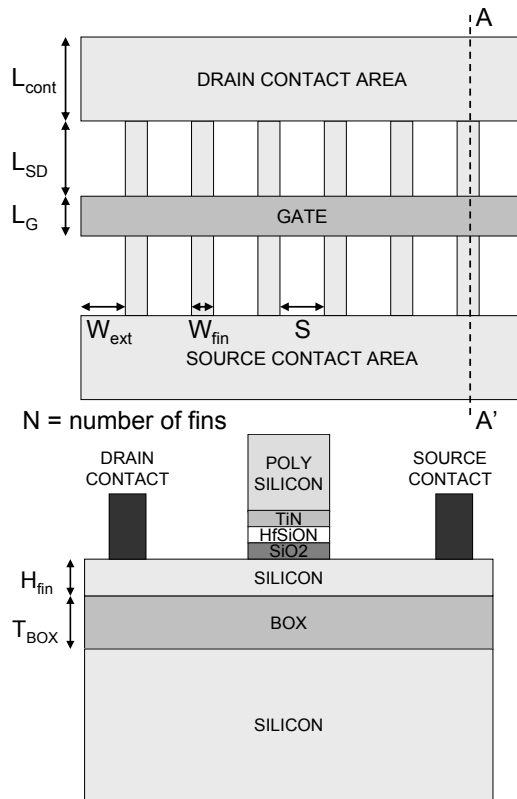
Figure 1: Horizontal (top) and vertical along cut-line A-A' (bottom) layout view of a FinFET device indicating the different geometrical parameters.
