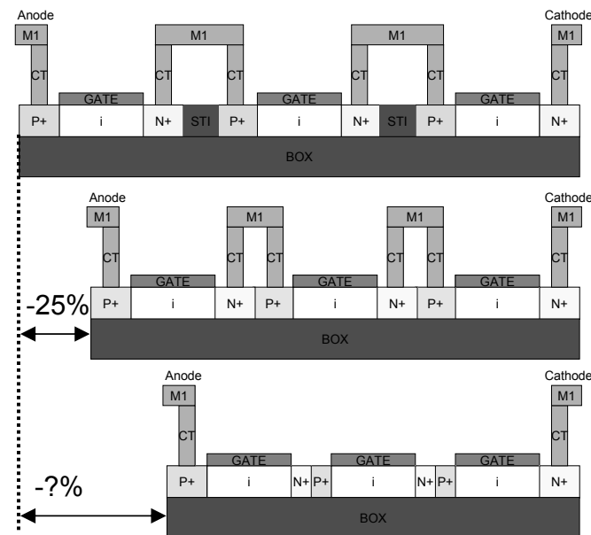
Figure 2: Cross-section of three gated diodes placed in series. The top figure shows separate devices, while in the middle the intermediate anodes and cathodes are merged into a single active area and are shorted by silicidation and the backend. By relying solely on the silicidation connection, the intermediate CTs and M1 can be removed resulting in a further layout reduction (bottom).
