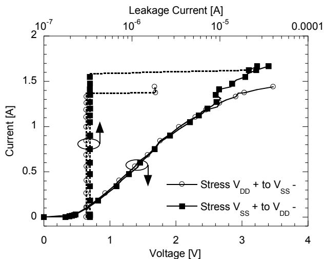
Figure 11: TLP measurements of the bidirectional FinFET power clamp, using a PMOS as BigFET.
