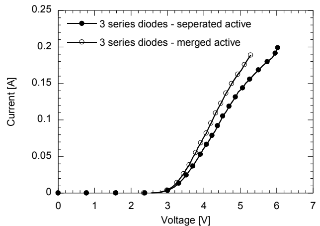
Figure 3: TLP-IV measurements for three diodes in series using different layout configurations. The diodes have 80 nm L_g and consist of 400 fins of 20 nm W_{fin} .
