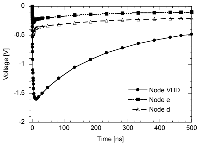
Figure 10: 1 kV HBM simulations of the circuit in Figure 9. HBM stress was applied negative between V_{DD} and V_{SS} .
