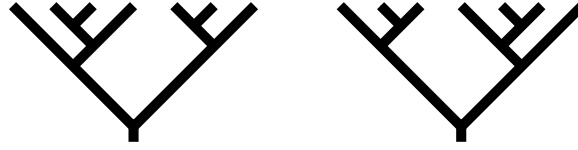
Figure 6: A planar binary tree with 6 inner vertices, and its image by reversal.
