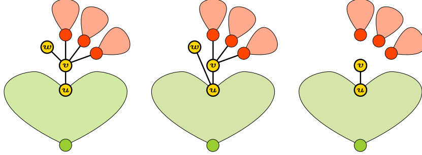
Figure 3: From left to right: T \curvearrowright_v w , T \curvearrowright_u w and S under T_1, \dots, T_k .
