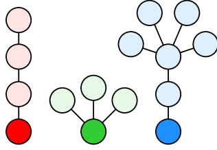
Figure 1: Linear tree \text{Lnr}_4 , corolla \text{Cr}_13 and fork \text{Frk}_{3,4} .
