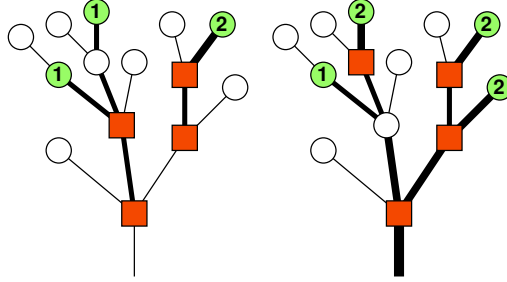
Figure 2: Two flows of size 4, on the same rooted tree with 14 vertices. Only the left one is closed.
