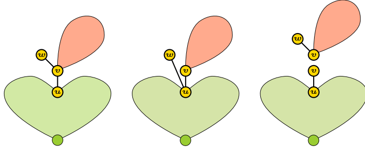
Figure 4: From left to right: T \curvearrowright_v w , T \curvearrowright_u w and S under S' .
