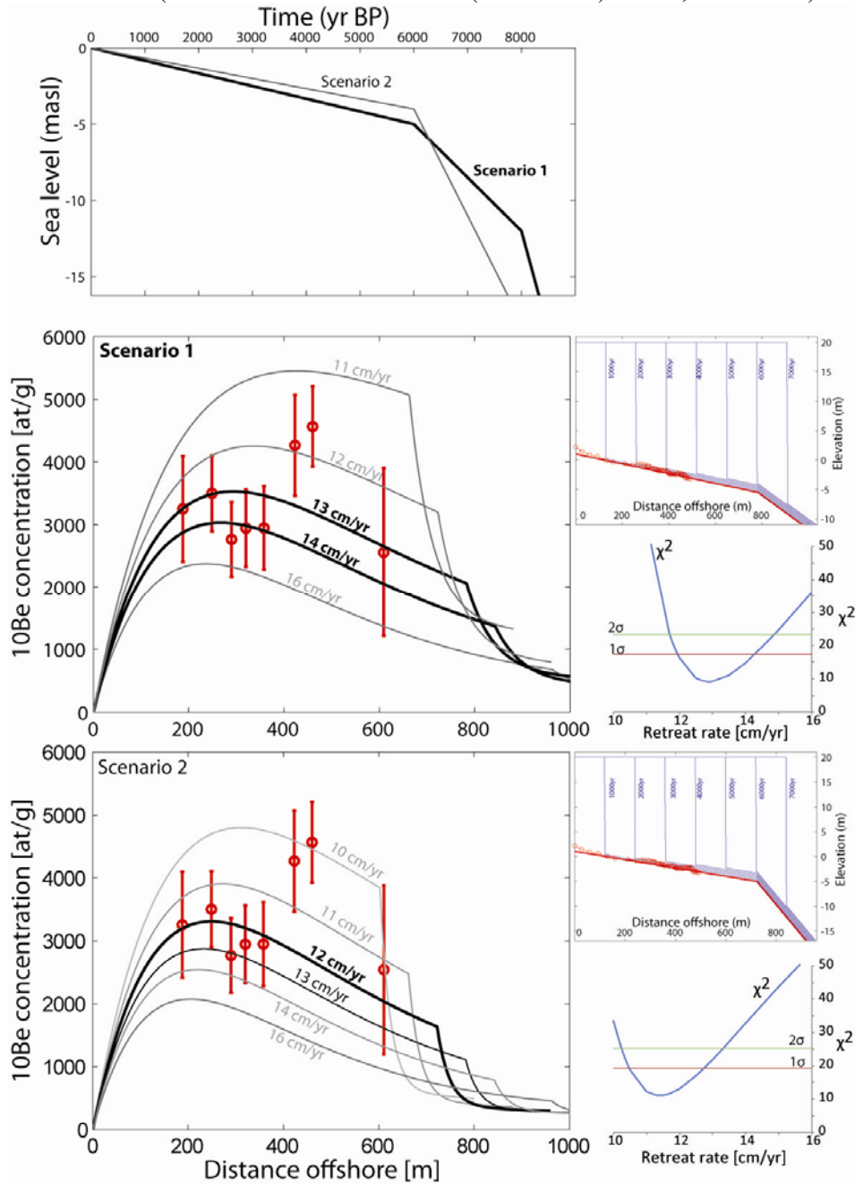
Figure 8. ^{10}\text{Be} concentrations in platform samples vs. distance from the cliff, and models of ^{10}\text{Be} profiles. A. 2 sea level rise scenarios from Massey et al. (2008) and Lambeck et al. (1997), respectively. B. The predicted ^{10}\text{Be} concentration curves are plotted for different long term cliff retreat rates according to sea level rise scenario 1. To the right, top inset displays the different topographic/bathymetric profiles (at 1000 yr intervals), and the fit to the platform GPS profile (circles). The platform lowering rate is chosen to assure that the fit of the final observed profile is optimized (see text, eqn. 16). Bottom inset show the \chi^2 metric of quality of fit. The best-fit value ( \chi^2 minimum value) is 12.8 cm/yr ( \chi^2=9.2 ). Corresponding 1\sigma (68%) and 2\sigma (95%) confidence intervals are, respectively, [11.9-14.3 cm/yr] and [11.7-14.9 cm/yr]. C. Same as B for scenario 2. Corresponding best fit, 1\sigma (68%) and 2\sigma (95%) confidence intervals are, respectively, 11.4 cm/yr ( \chi^2=11.0 ), [10.5-12.7 cm/yr] and [10.2-13.3 cm/yr].
