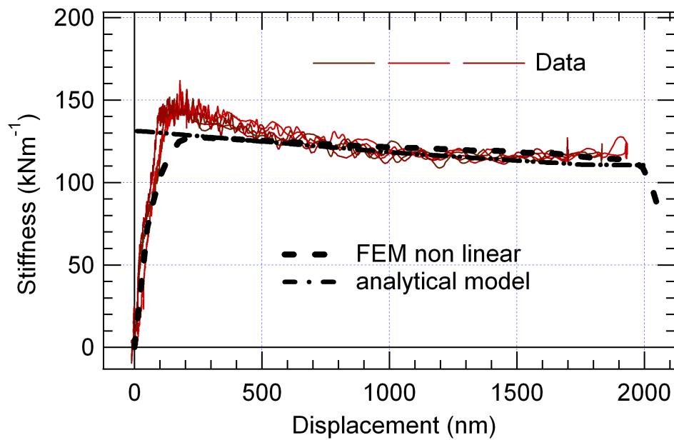
Figure 6: Stiffness vs. displacement curves of experiments compared to theoretical and FEM results taking into account the non linear elasticity of silica [8]
