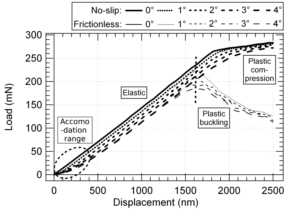
Figure 4: FEM load/displacement calculation of misalignment effects between the indenter tip and top of the pillar under two contact conditions (no-slip or frictionless)
