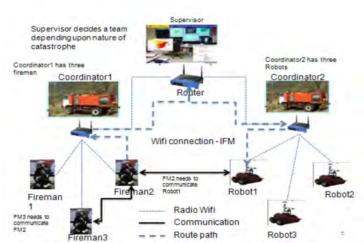
Figure 3: ROSACE Communication
