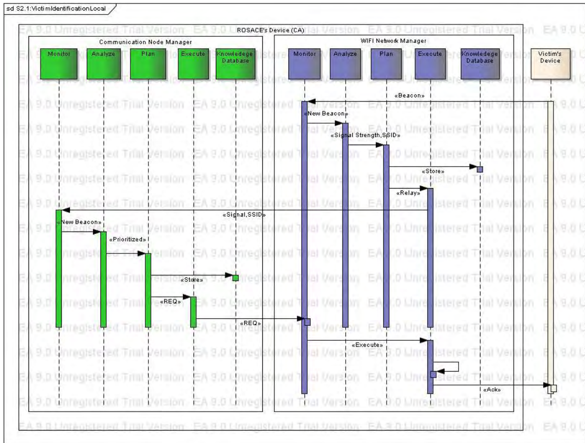
Figure 9.22: Sequence diagram for tracing beacon from the victim's device
