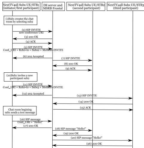
Fig. 5: Virtual Chat Room Call Flow
