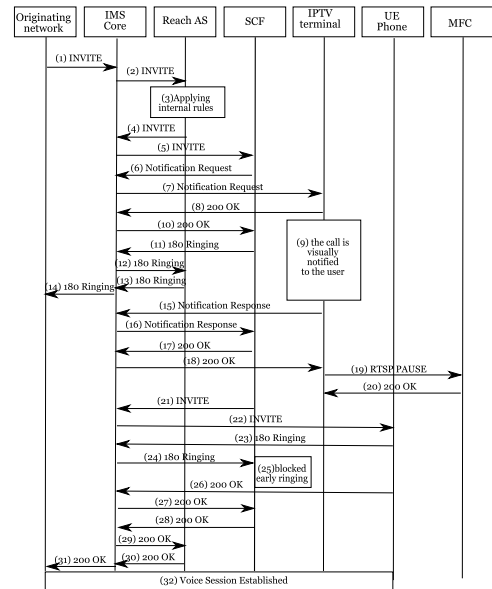
Fig. 4: Incoming Call Management Call Flow (accepted call)
