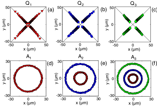
FIG. 6 (color online). Upper row: electrically-controlled radial position in the (x, y) plane of quadrupoles Q_1 ( \blacktriangledown ), Q_2 ( \blacksquare ), and Q_3 ( \blacklozenge ) for a x -polarized incident illumination at \lambda = 532 nm, \tilde{U} being varied from 1 to 1.6. Bottom row: polarization-controlled azimuthal position of the m quadrupoles embedded in the bright field array A_m when the angle \alpha between the direction of the pair of parallel linear polarizers and the x axis is varied from 0 to \pi . Quadrupoles labeling is the same as above.
