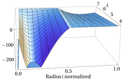
Fig. 4. Numerical test of the conditions of Proposition 5.
