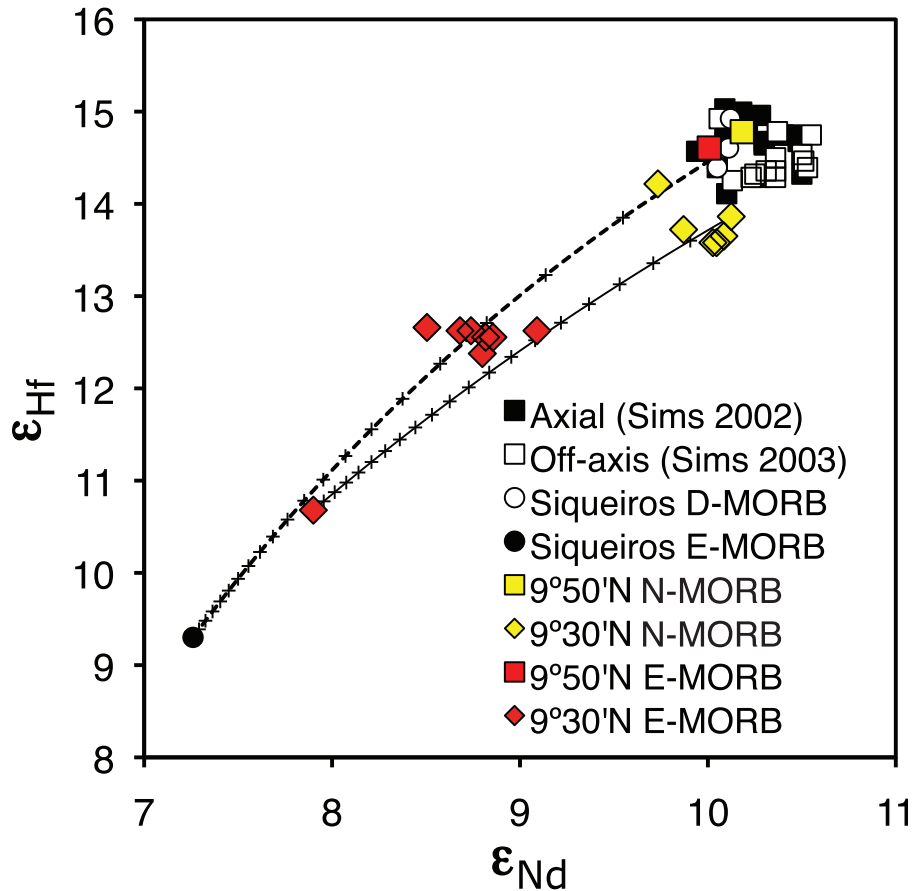
Fig. 5. \epsilon_{Nd} vs \epsilon_{Hf} for 9–10°N East Pacific Rise lavas. The dashed line is a binary mixing curve between Siqueiros E-MORB and D-MORB. The continuous line is a binary mixing curve between 9°30'N N-MORB (sample 2706-7) and E-MORB (sample 2703-1). Data sources and symbols are the same as in Fig. 2. Additional Siqueiros isotope data are from Sims et al. (2002). (See text for discussion.)
