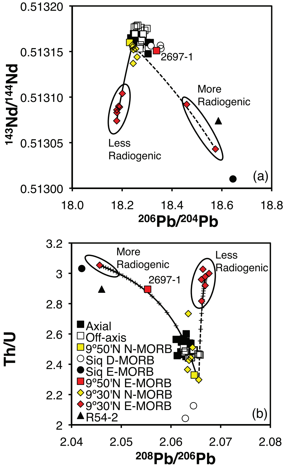
Fig. 7. Variation of (a) ^{206}\text{Pb}/^{204}\text{Pb} vs ^{143}\text{Nd}/^{144}\text{Nd} and (b) ^{208}\text{Pb}/^{206}\text{Pb} vs Th/U. Mixing lines are designated by a dashed line between samples 2706-7 (depleted end-member) and 2703-1 (more radiogenic E-MORB Pb end-member) and a continuous line between 2706-7 and 2489-3 (less radiogenic E-MORB Pb end-member). It should be noted that both E-MORB end-members are more isotopically enriched than N-MORB with respect to ^{143}\text{Nd}/^{144}\text{Nd} . Data sources and symbols are the same as in Figs 2 and 5, and 6.
