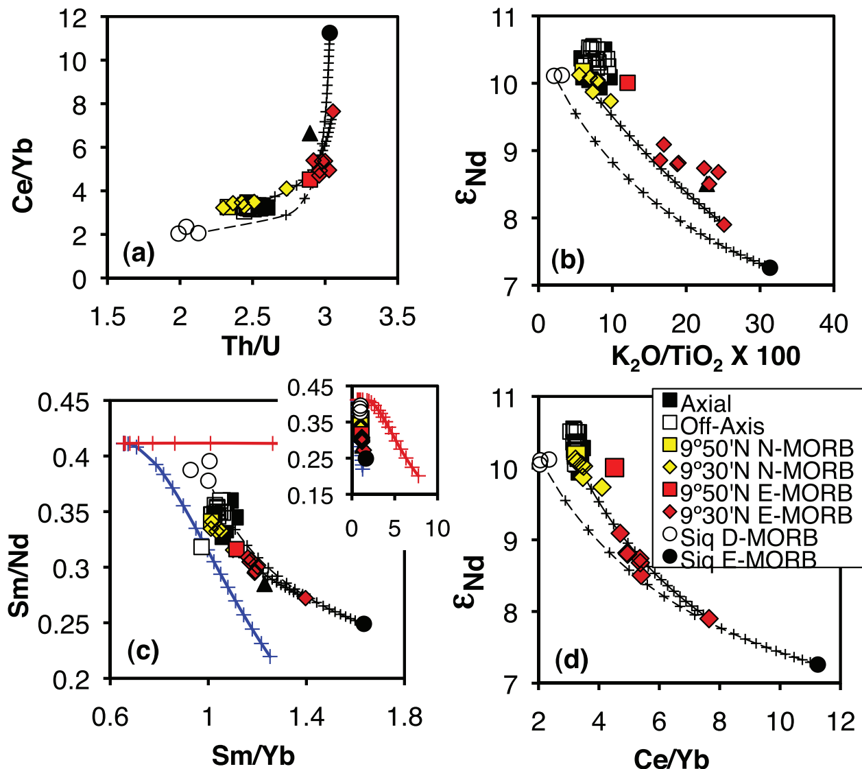
Fig. 4. Variation of (a) Th/U vs Ce/Yb, (b) K_2O/TiO_2 \times 100 vs \epsilon_{Nd} , (c) Sm/Yb vs Sm/Nd, and (d) Ce/Yb vs \epsilon_{Nd} for 9^\circ N East Pacific Rise lavas. The dashed black line is a mixing trajectory between Siqueiros D-MORB (A2384-6) and E-MORB (A2390-5) end-members (Perfit et al. , 1996; Lundstrom et al. , 1999; Sims et al. , 2002). The continuous black line is a mixing trajectory between the most depleted (2706-7) and enriched (2703-1) samples from this study. Mixing increments of 5% are designated by black crosses. Also shown in (c) are modal accumulated fractional melting curves for garnet peridotite and spinel peridotite. Crosses on the melting trajectories indicate 0.1%, 1–10% in 1% increments, 12.5%, 15%, 17.5%, and 20–100% in 10% increments. (See text for details.) Inset is the same as (c) but at a different Sm/Yb scale to show the large extent of Sm/Yb fractionation by melting of garnet peridotite as compared with clinopyroxene-bearing spinel peridotite. The symbols and data sources are the same as in Fig. 2.
