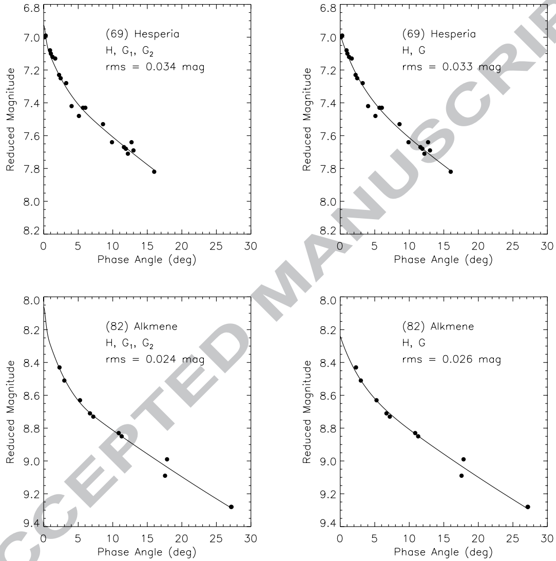
Fig. 3. As in Fig. 2 for the M-class asteroid (69) Hesperia and the S-class asteroid (82) Alkmene.
