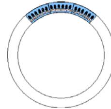
Figure 17: Generator architecture - A synchronous machine with radial flux and mounted surface magnets (only 3 pole pairs shown)
