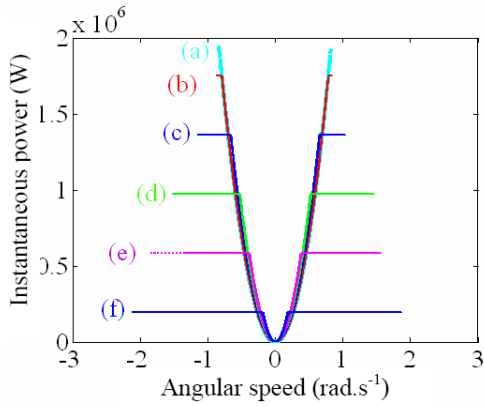
Figure 13: Point cloud of the instantaneous power vs. angular speed for several power leveling ratios - (a: \alpha=1 ), (b: \alpha=0.9 ), (c: \alpha=0.7 ), (d: \alpha=0.5 ), (e: \alpha=0.3 ), (f: \alpha=0.1 )
