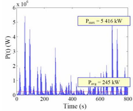
Figure 16: Recovered power with latching control
