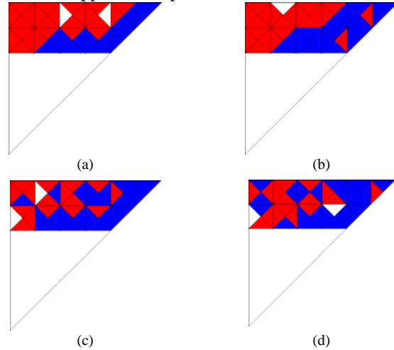
Fig. 8. Optimal material distributions after 200 generations for pX=0.1 and (a) pM=0.3, (b) pM=0.5, (c) pM=0.7 and (d) pM=0.9
