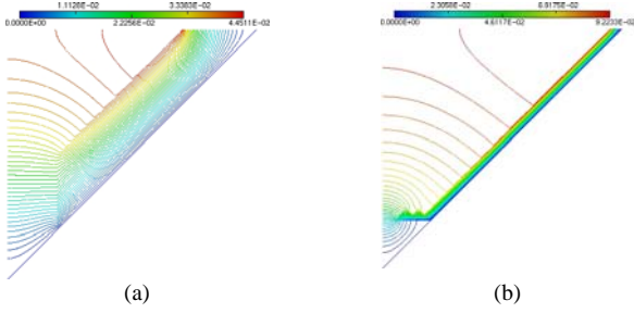
Fig. 15. Corresponding flux density lines
