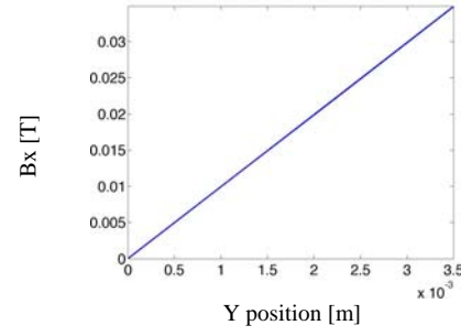
Fig. 7. Magnetic induction along [O, \alpha] for pX=pM=0.1
