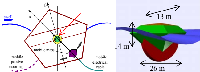
Figure 1b: Primary dimensions of the full scale SEAREV prototype design
